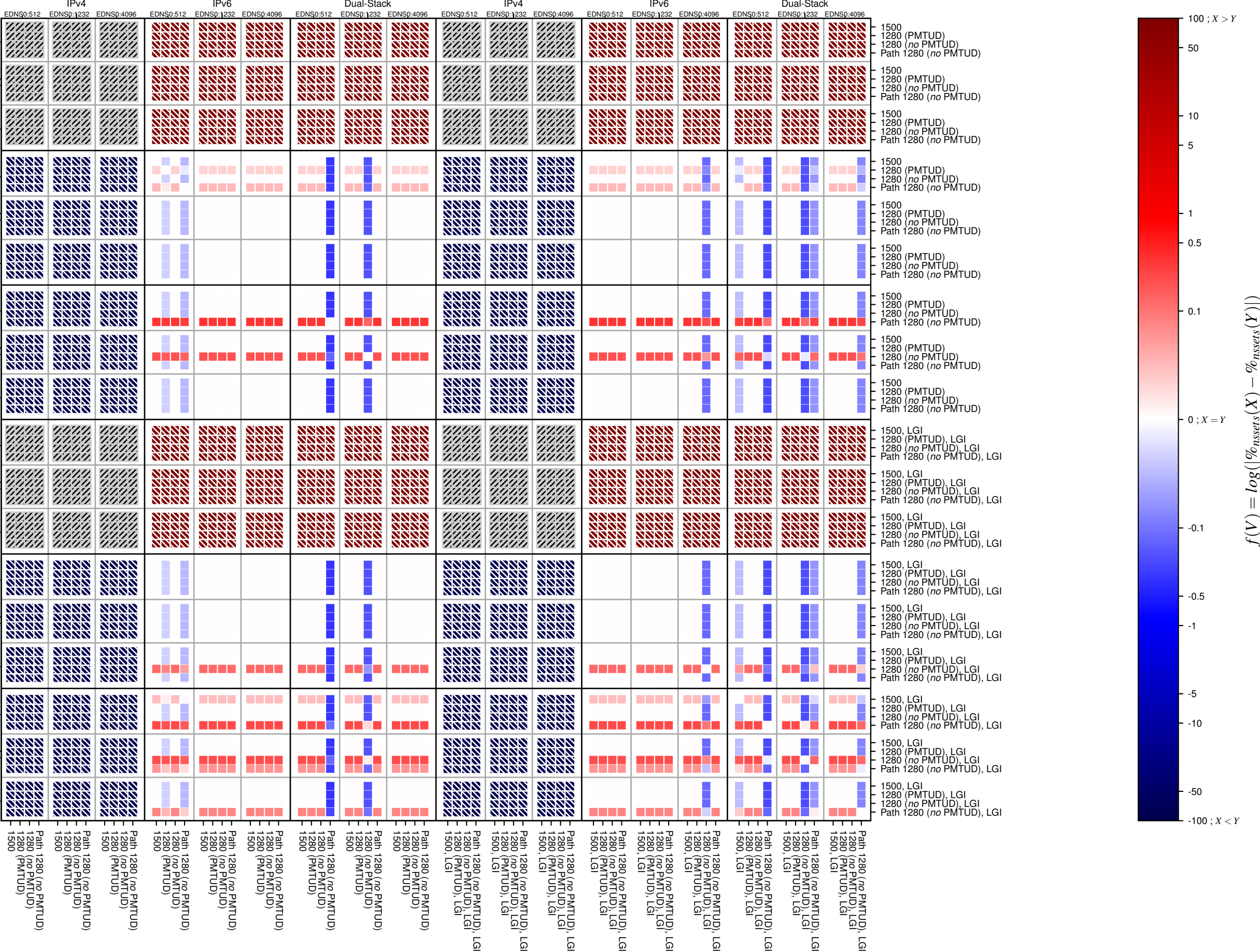
dnssec-v6-TCP_server_mss_ok
