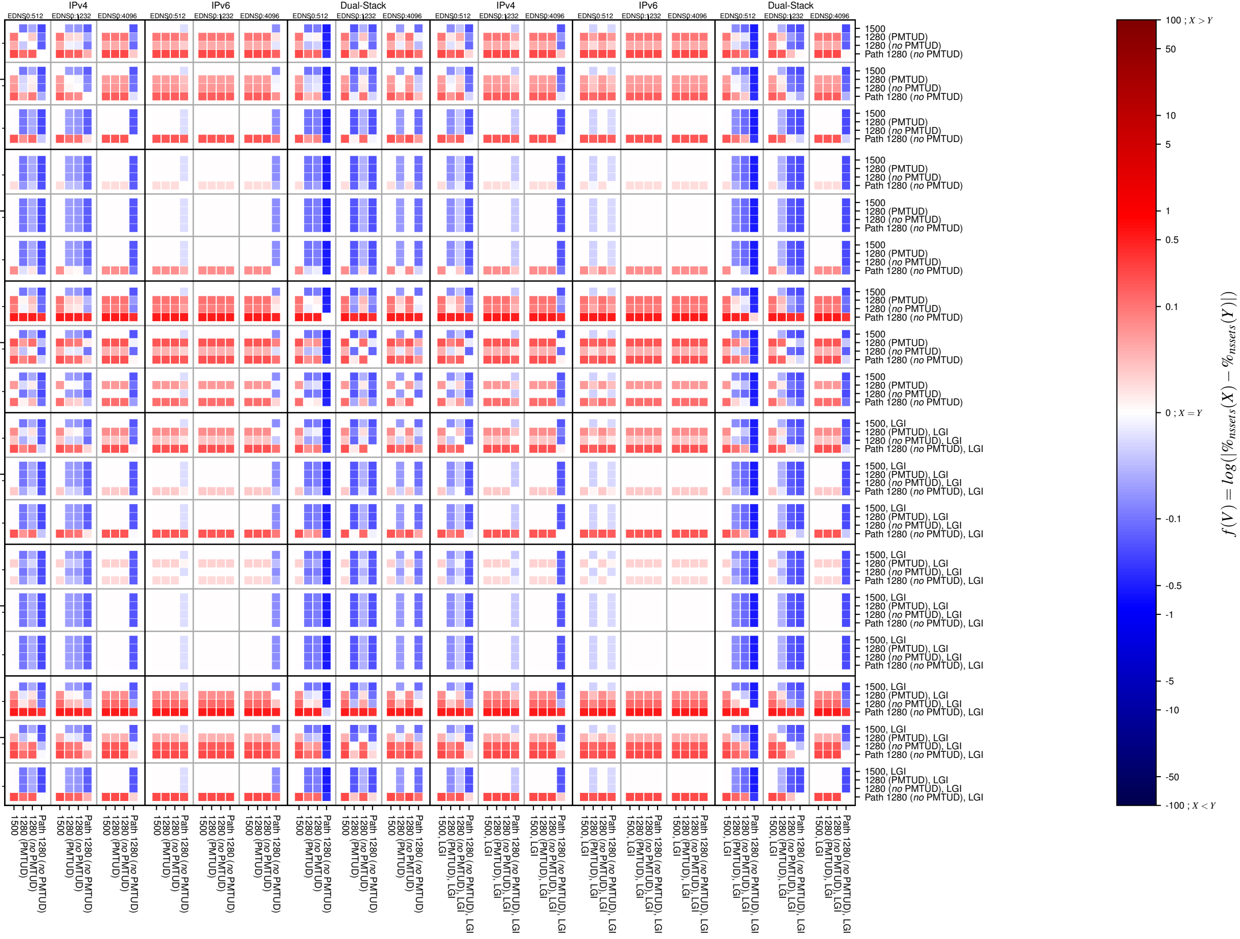
dnssec-both-TCP_server_mss_ok
