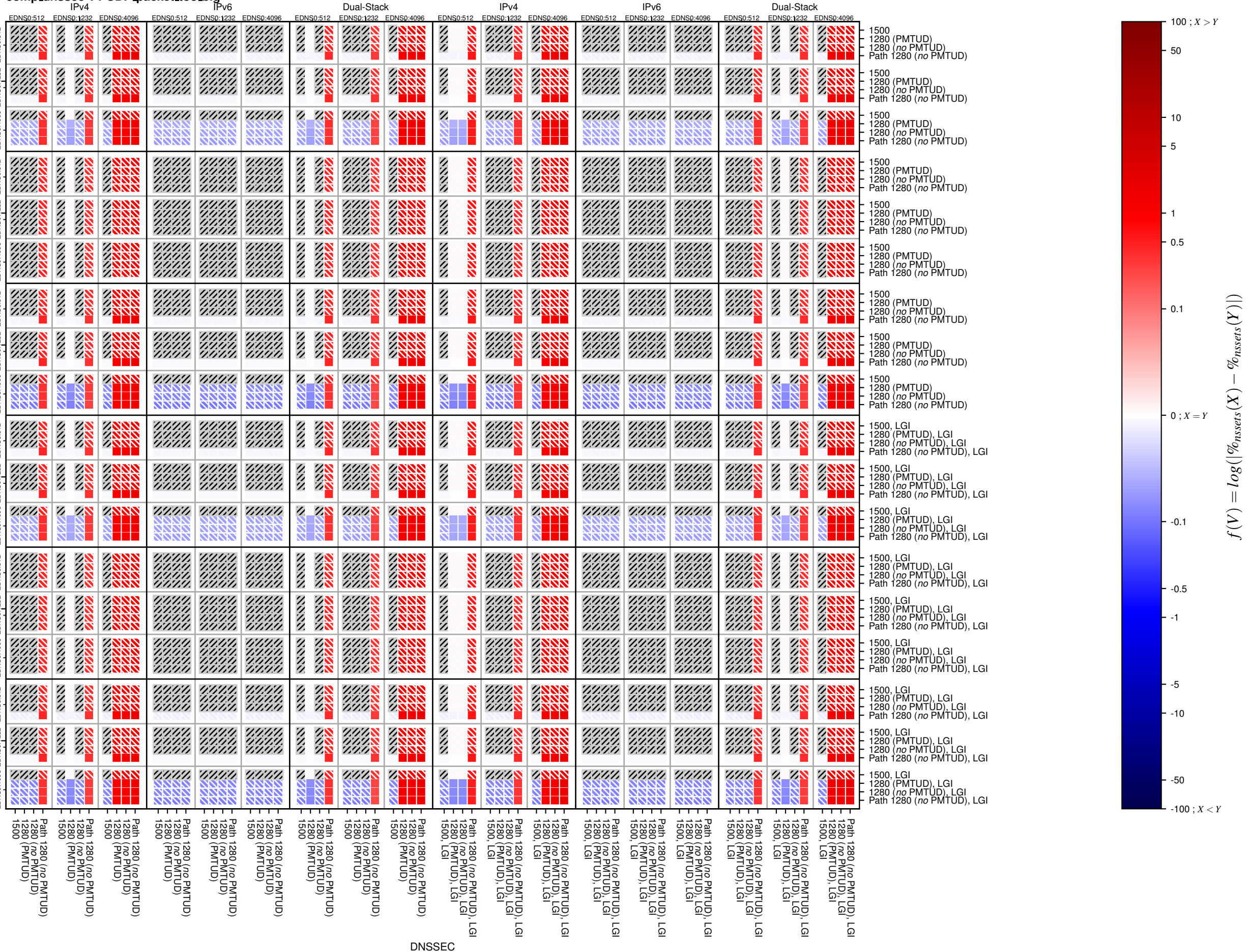
comp_dnssec-v4-UDP_packet_too_big
