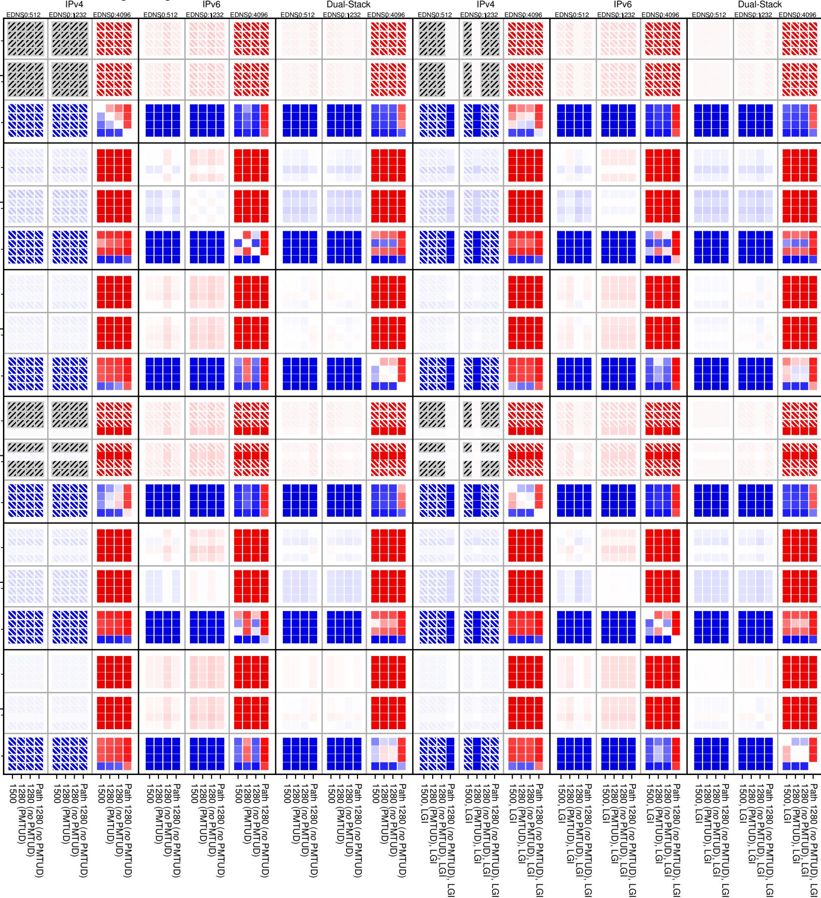
dnssec-both-UDP_frag_too_big
