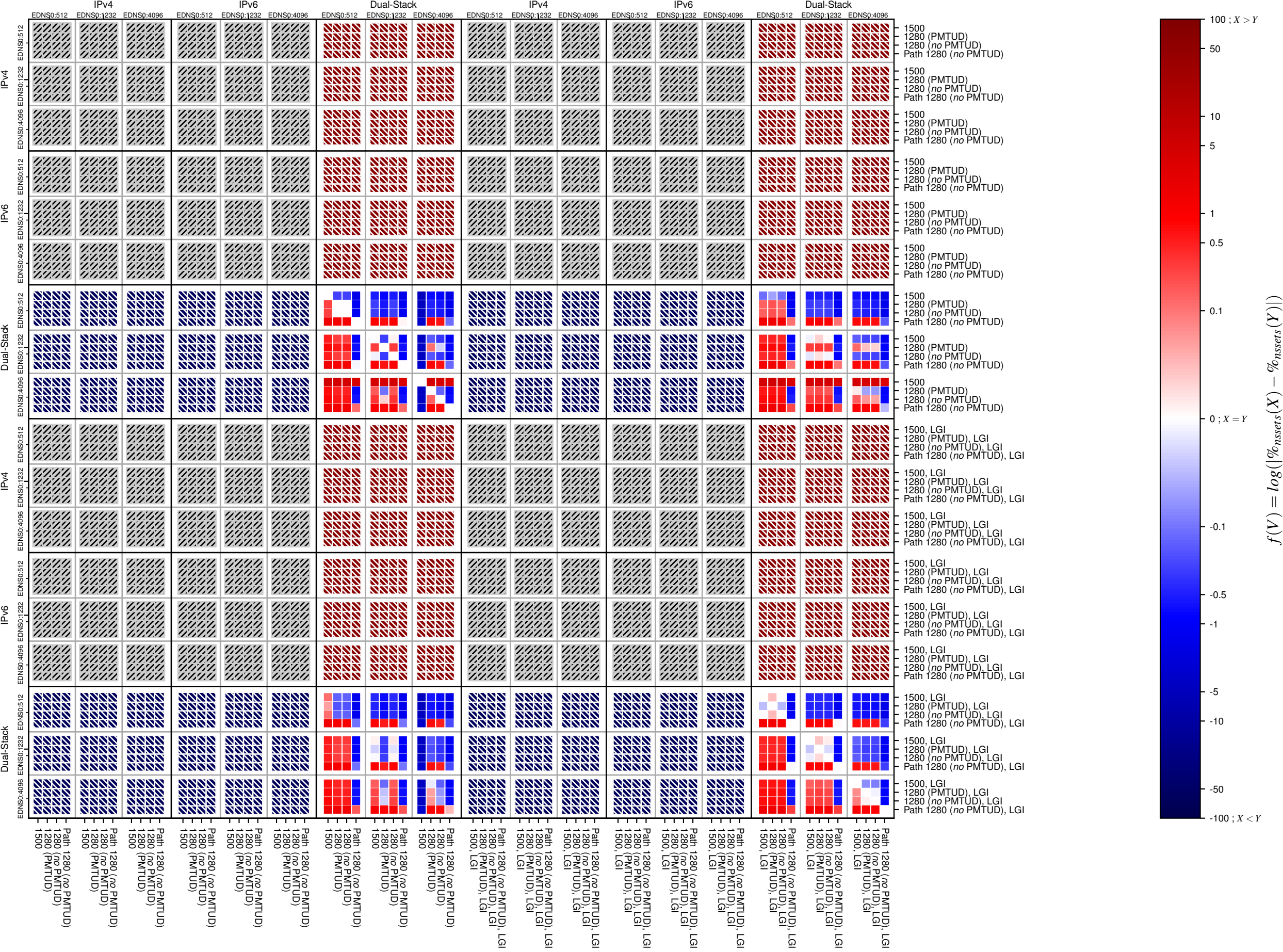
dnssec-v4-UDP_TCP_afi_count
