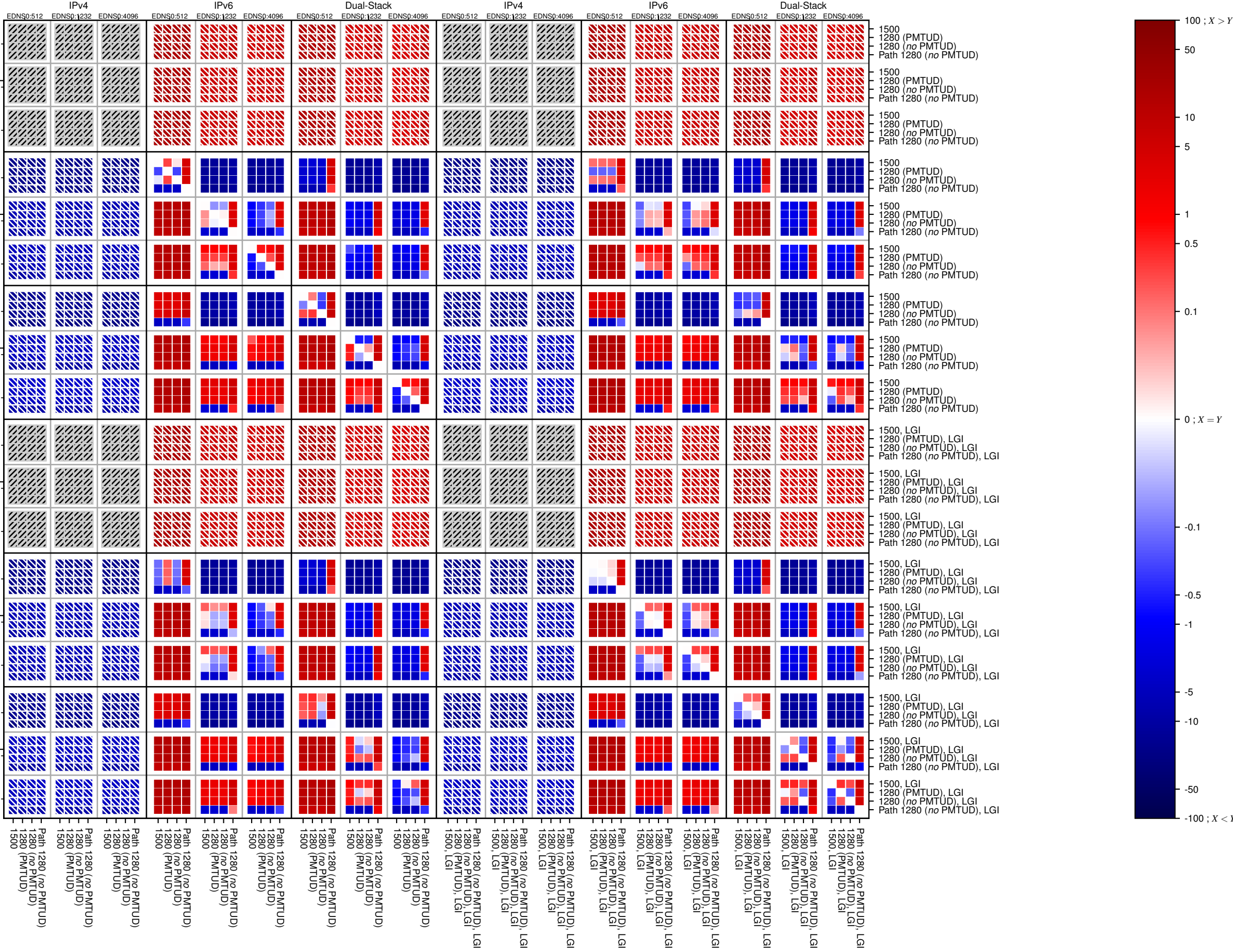
dnssec-v6-TCP_count
