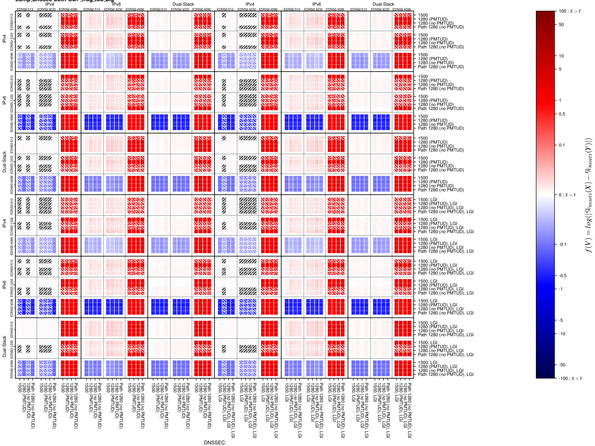
comp_dnssec-both-UDP_frag_too_big
