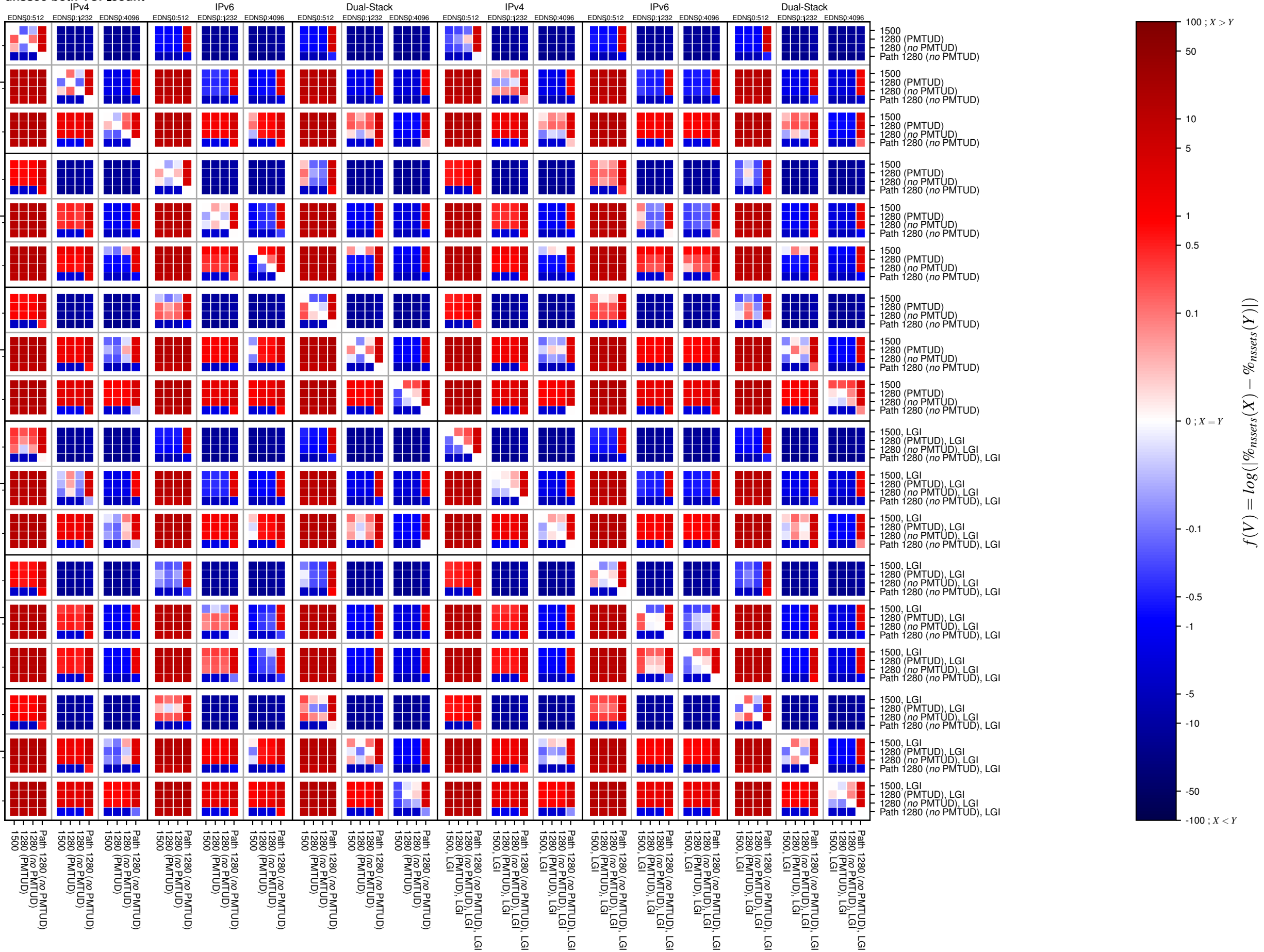
dnssec-both-TCP_count
