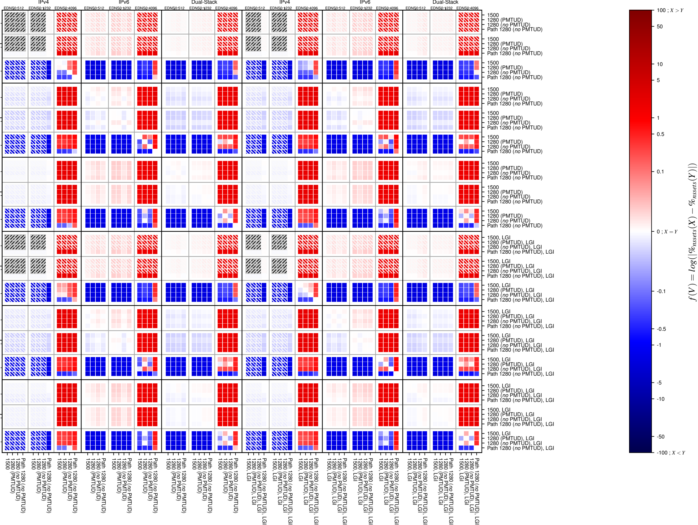
dnssec-both-UDP_frag_too_big
