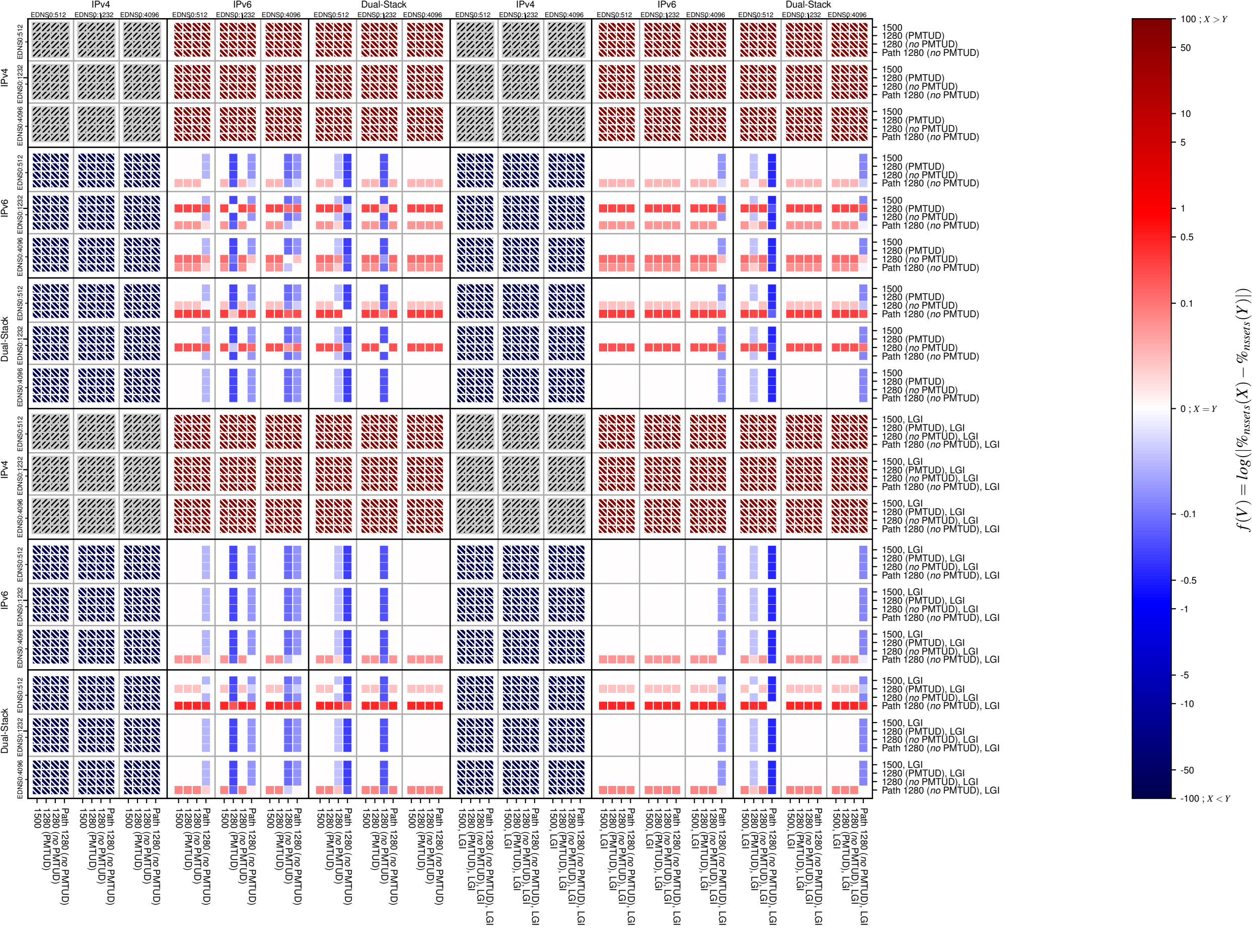
dnssec-v6-TCP_server_mss_ok
