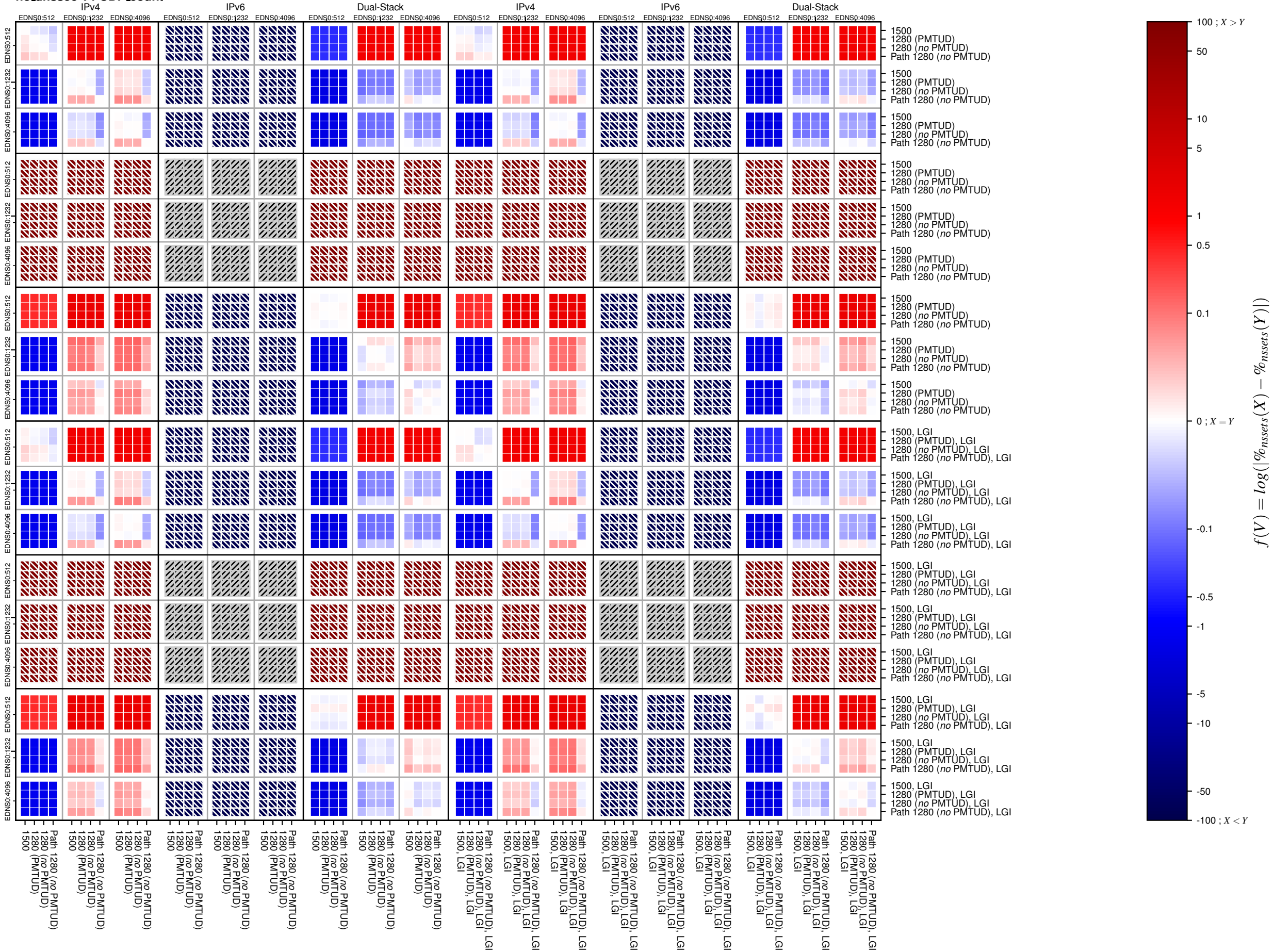
no_dnssec-v4-UDP_count
