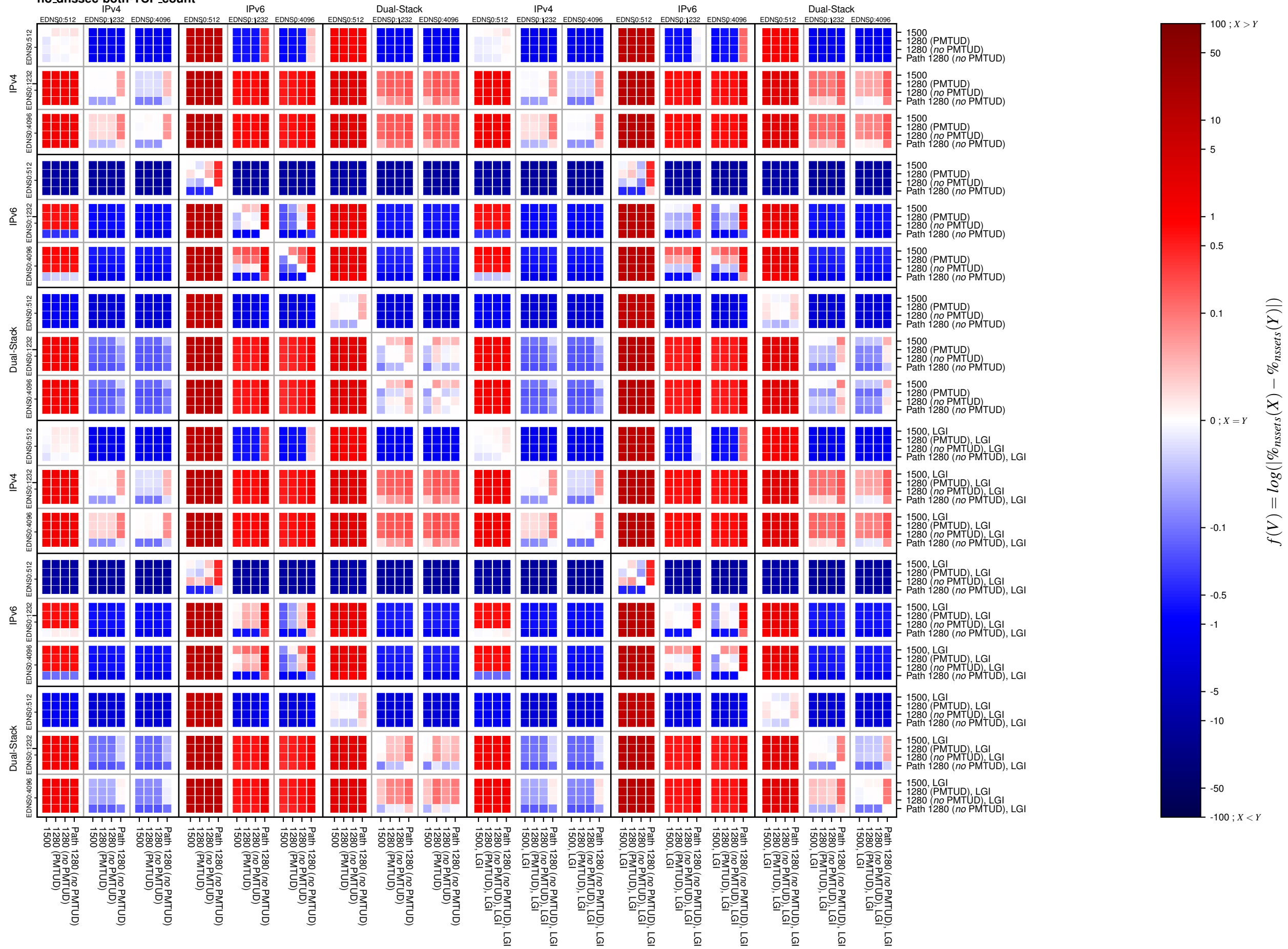
no_dnssec-both-TCP_count
