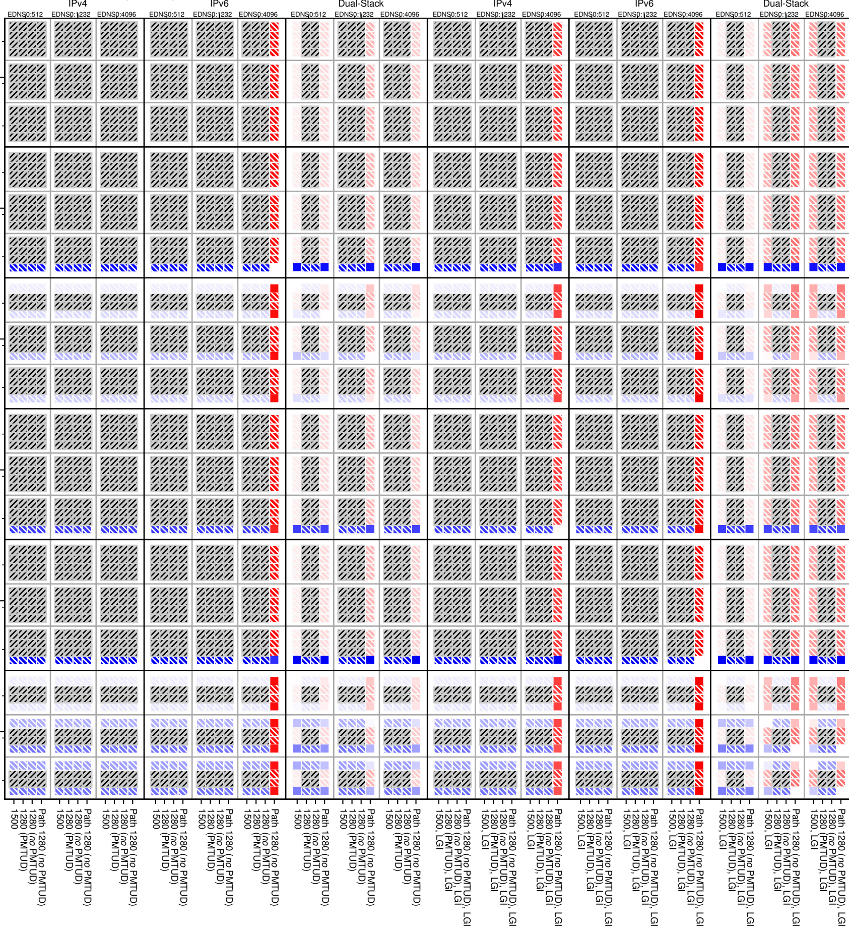
dnssec-both-TCP_frag_too_big
