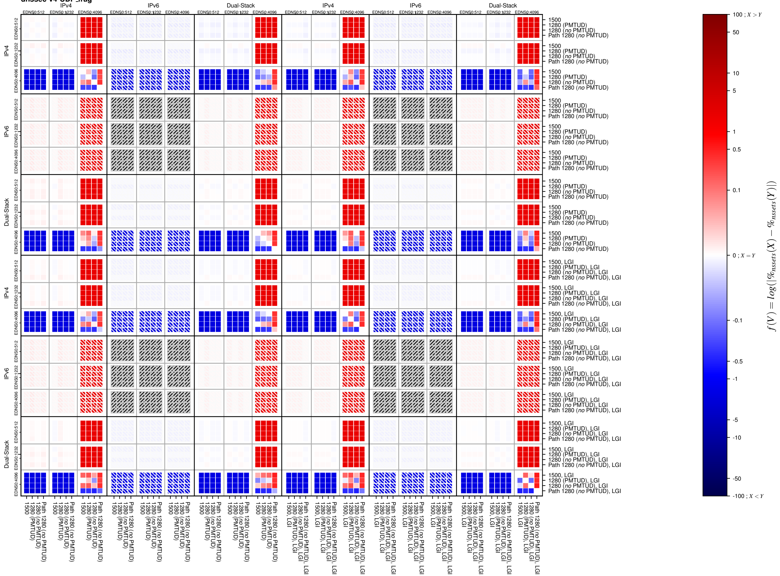
dnssec-v4-UDP_frag
