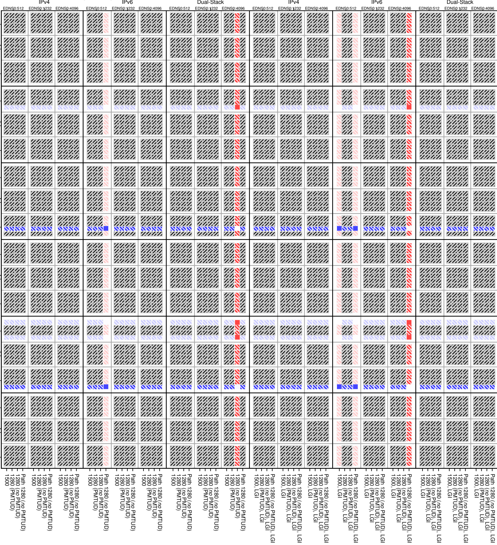
no_dnssec-both-TCP_frag_too_big
