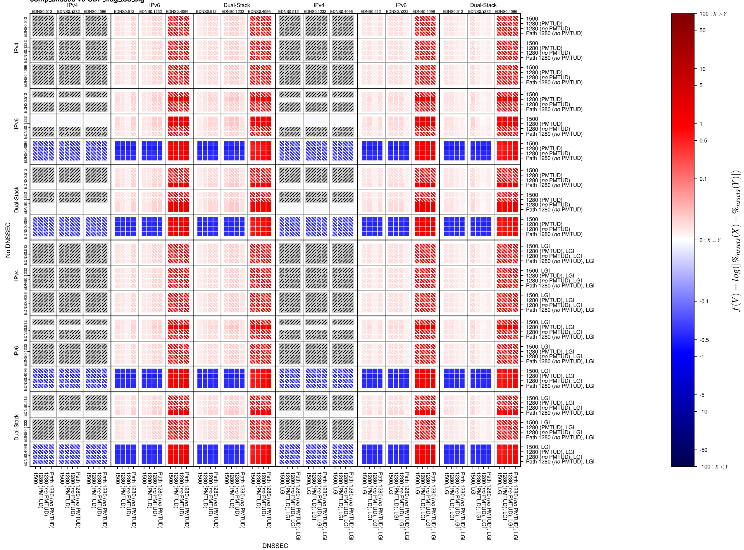
comp_dnssec-v6-UDP_frag_too_big
