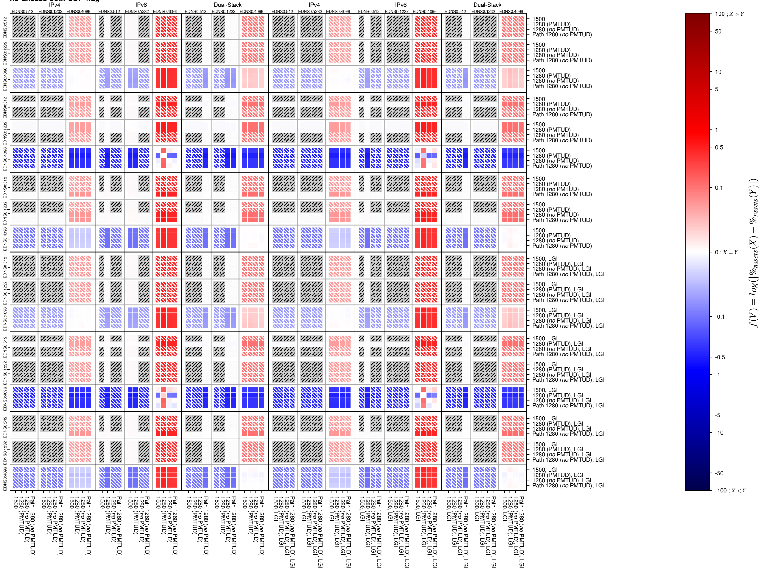
no_dnssec-both-UDP_frag
