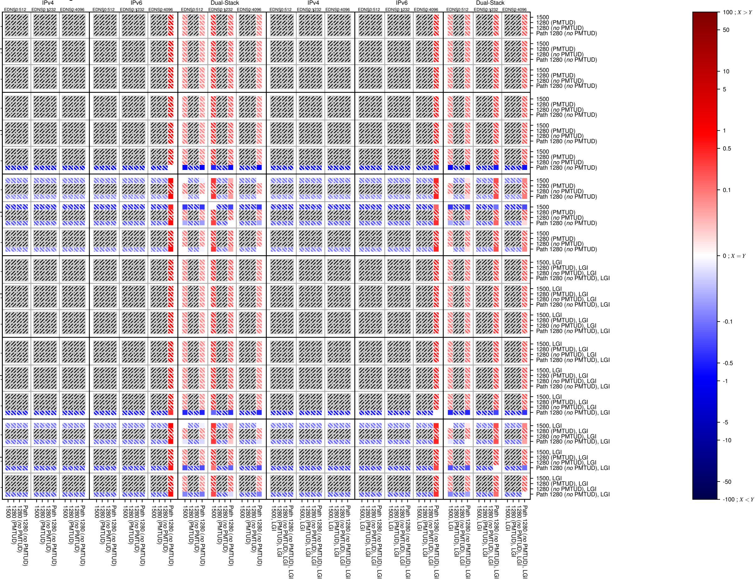
dnssec-v6-TCP_frag
