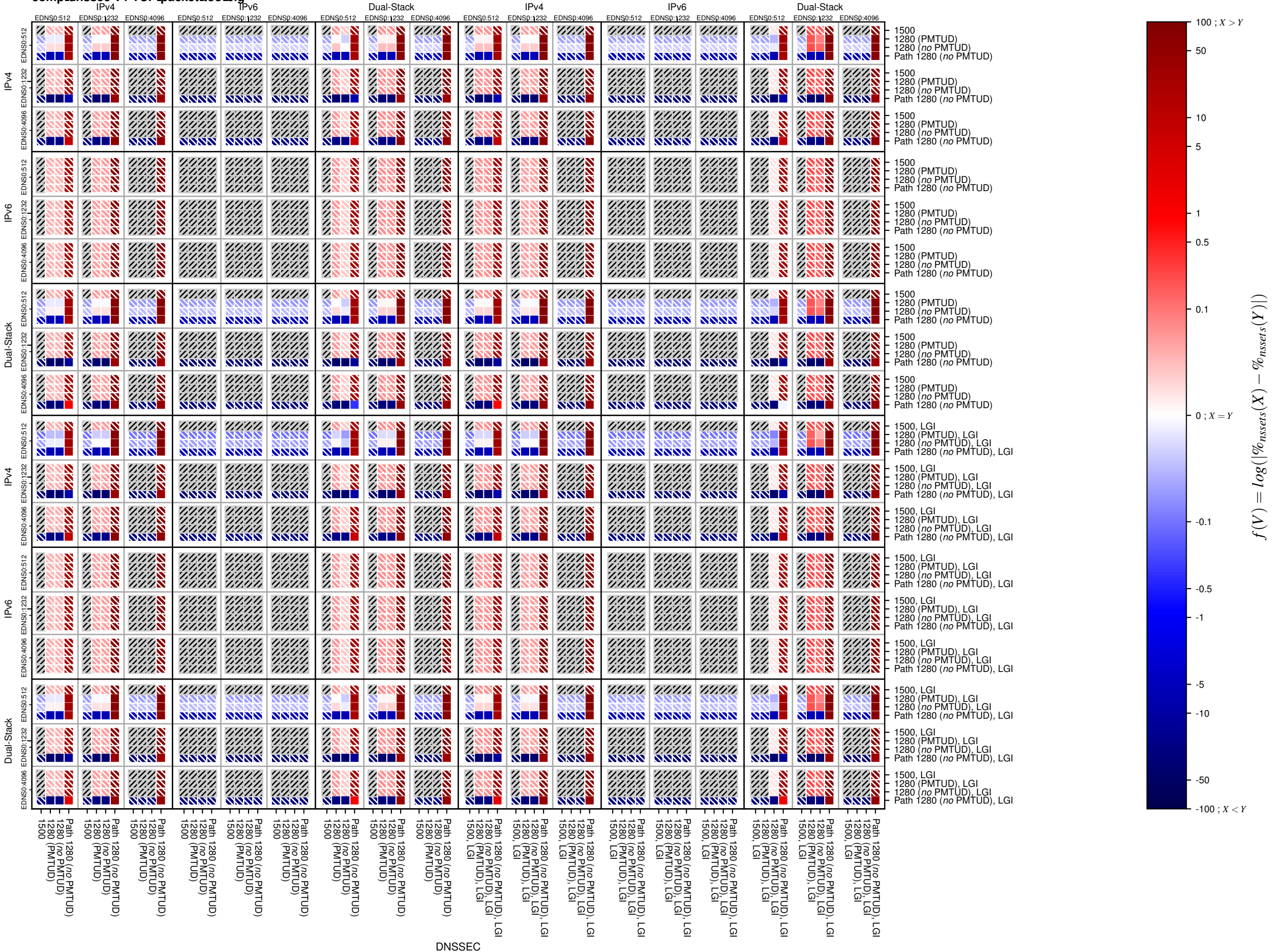
comp_dnssec-v4-TCP_packet_too_big
