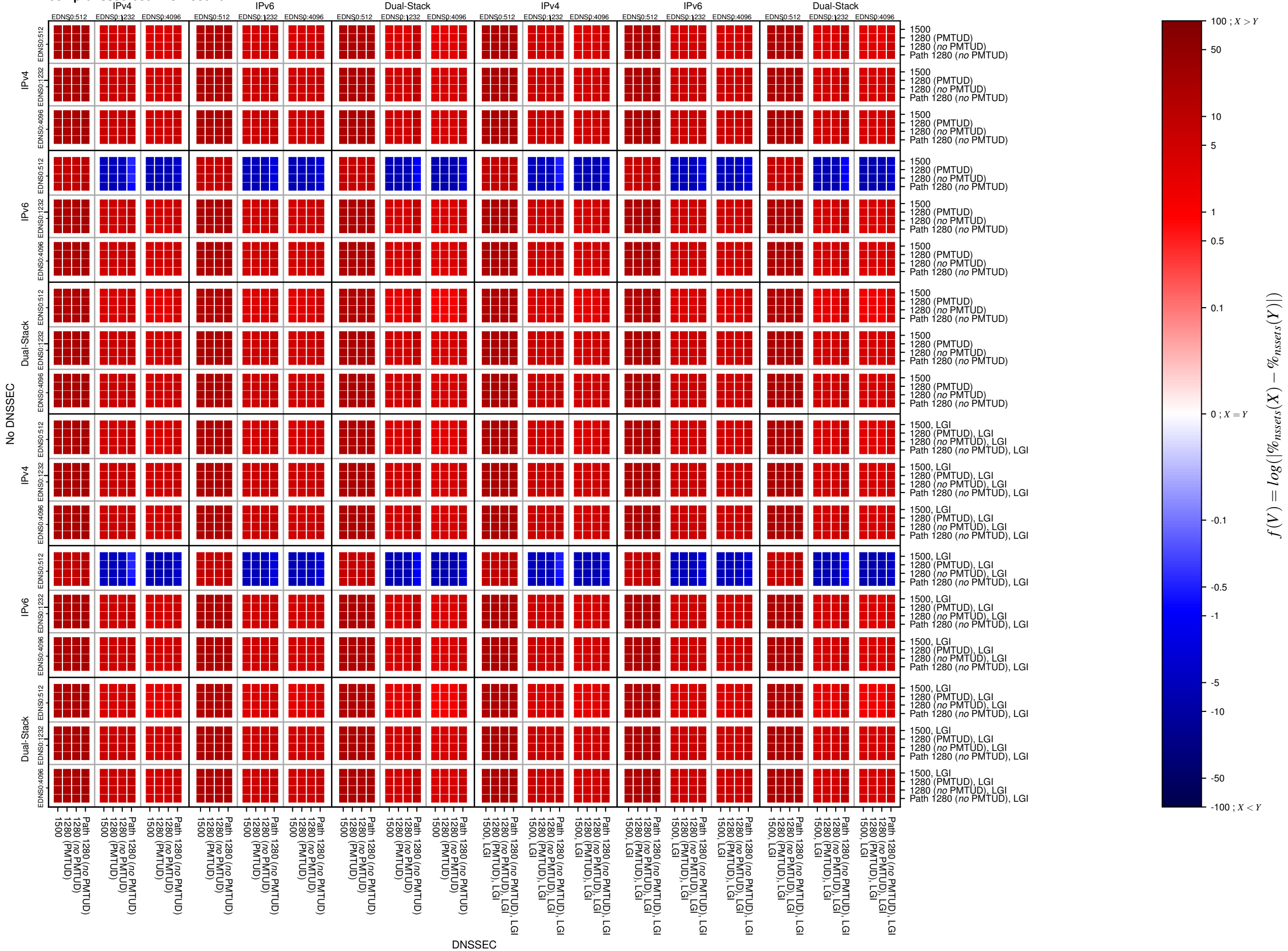
comp_dnssec-both-TCP_count
