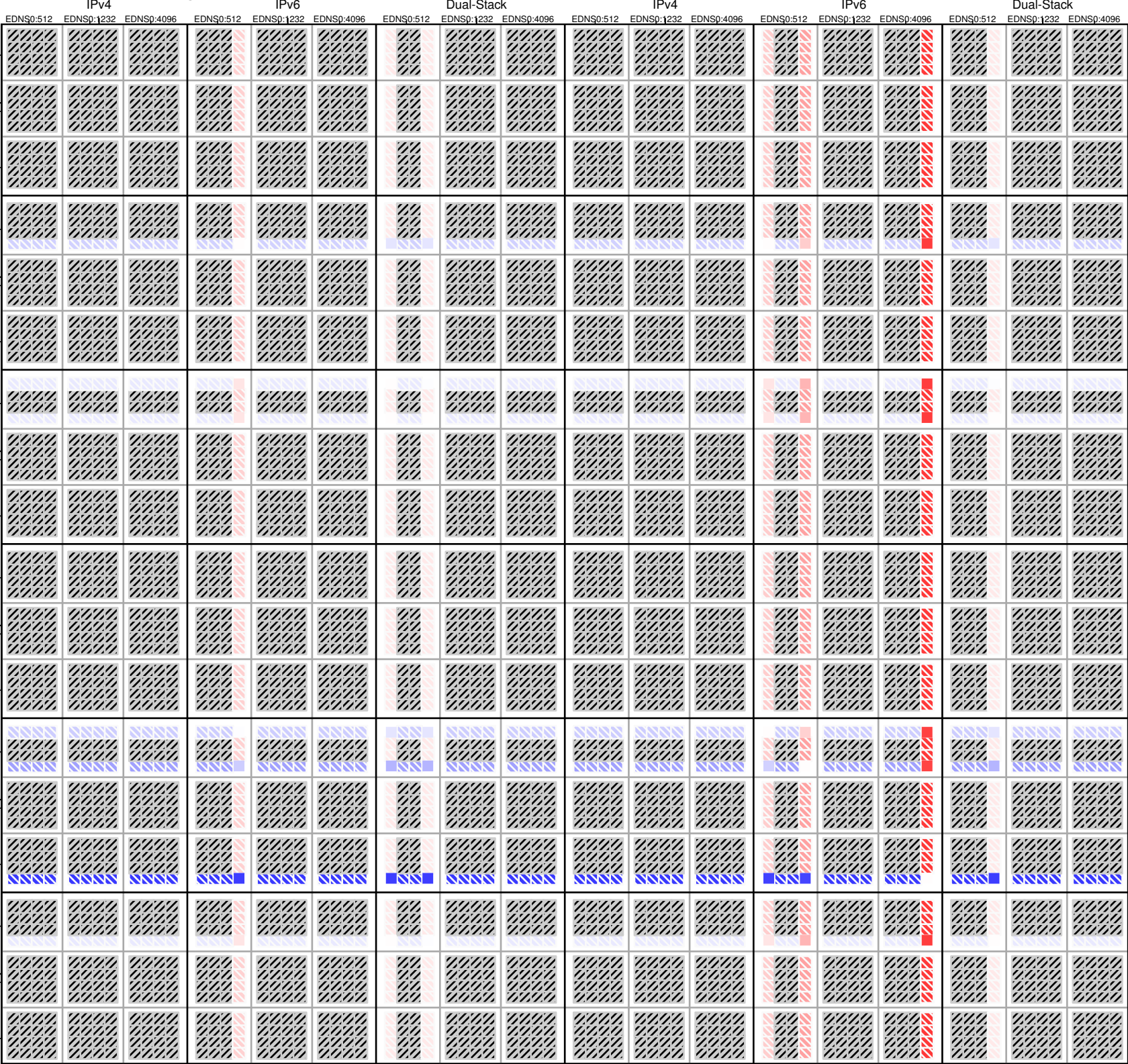
no_dnssec-both-TCP_frag
