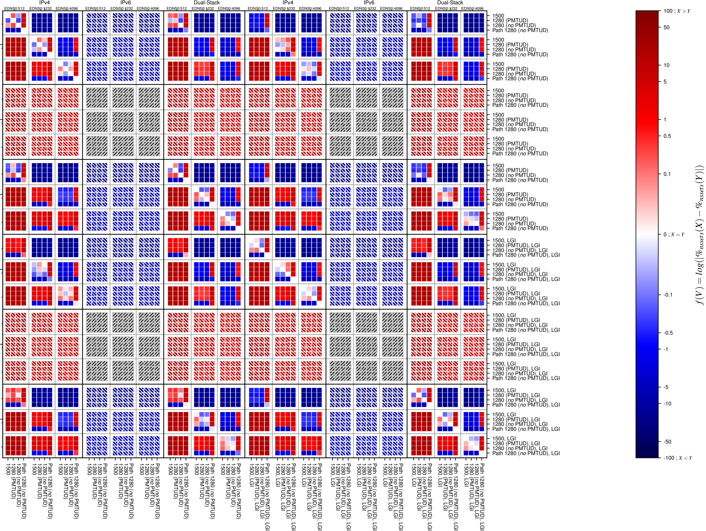
dnssec-v4-TCP_count
