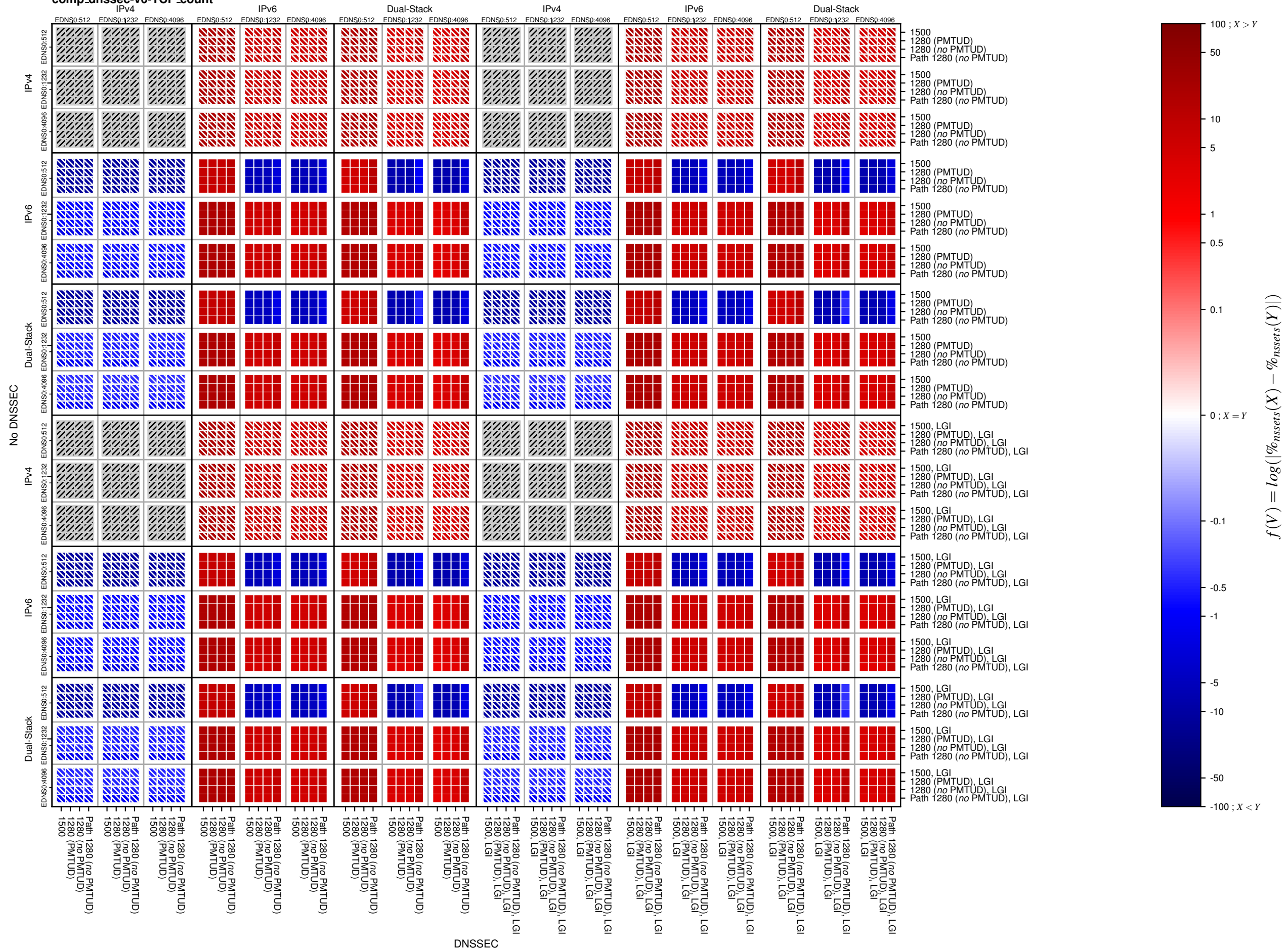
comp_dnssec-v6-TCP_count
