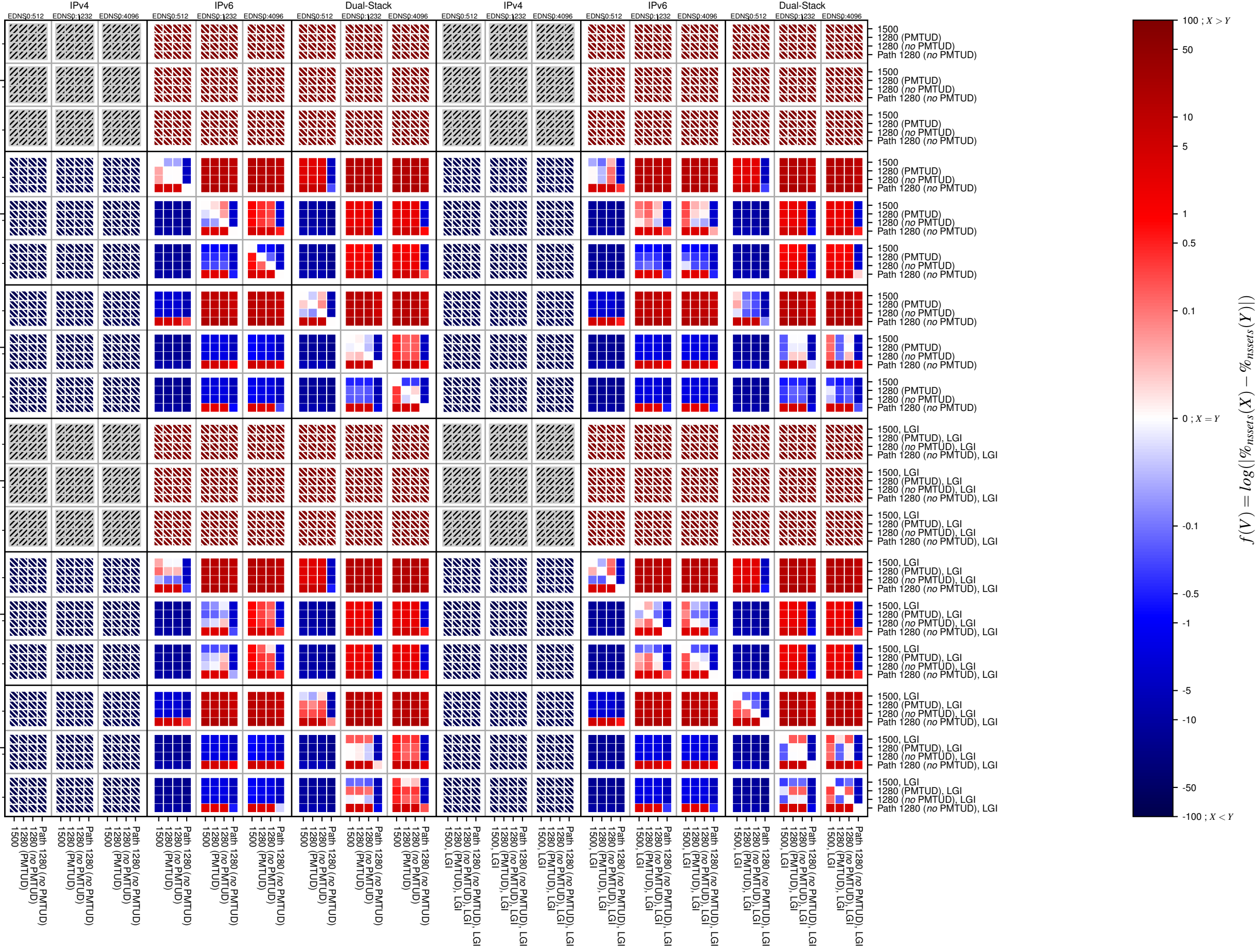
dnssec-v6-UDP_count
