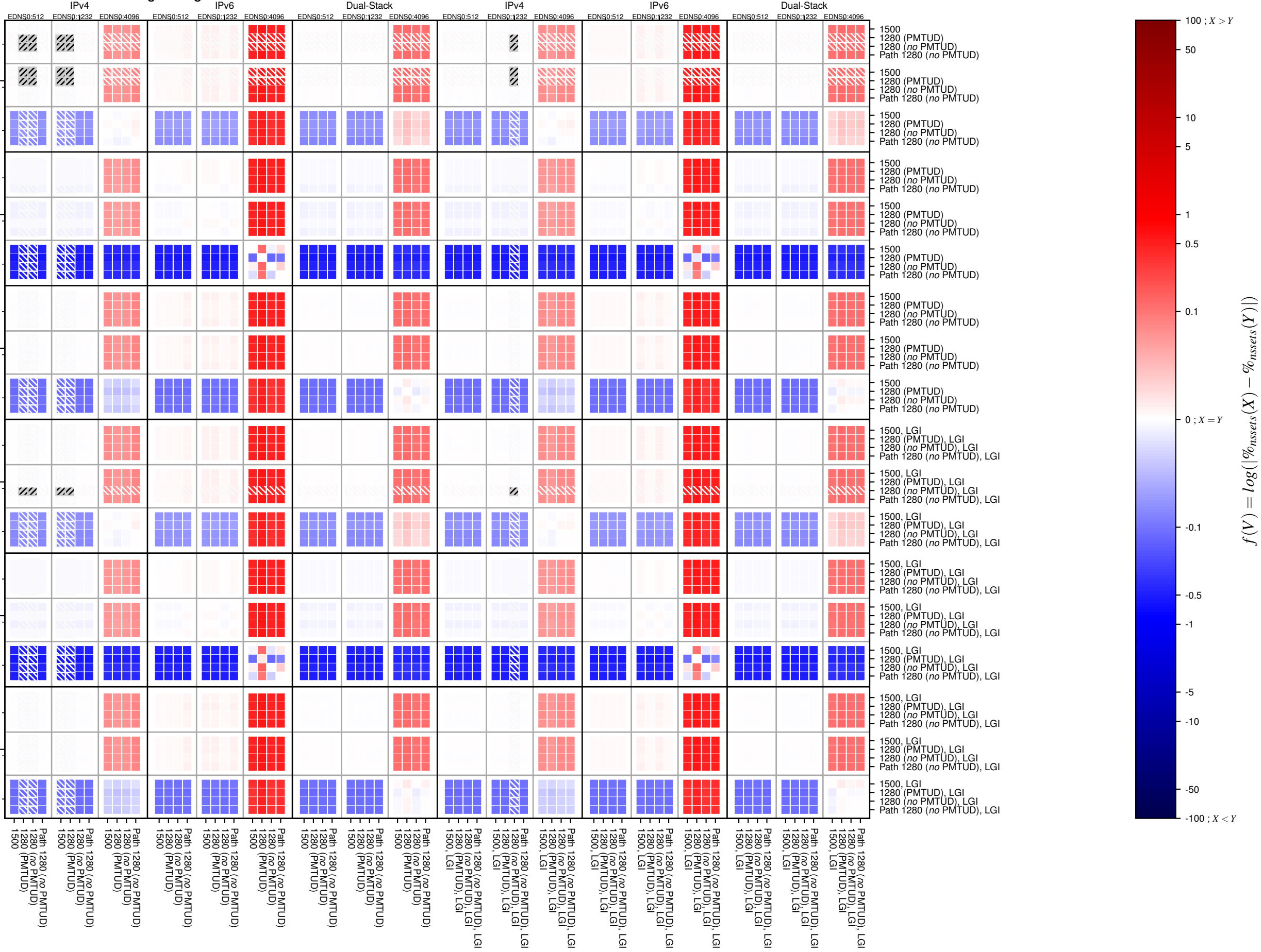
no_dnssec-both-UDP_frag_too_big
