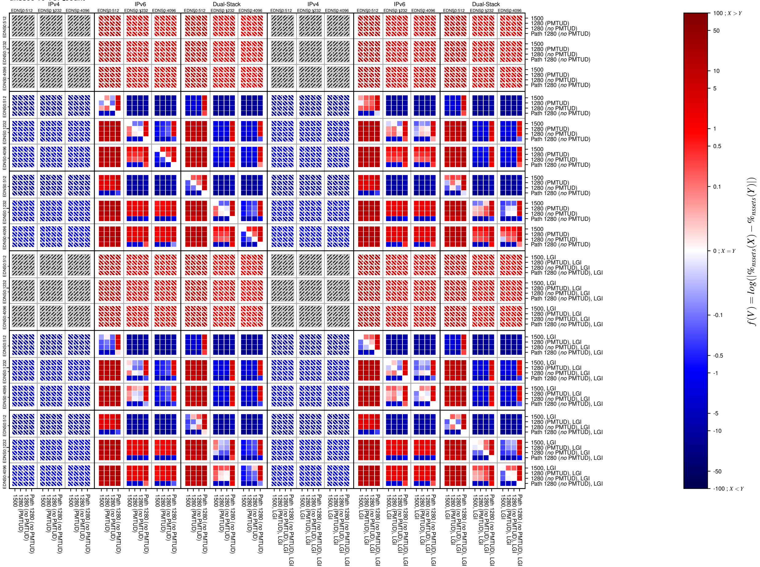
dnssec-v6-TCP_count
