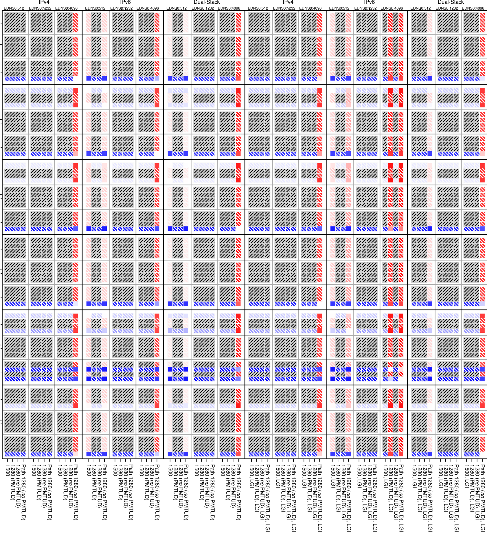
no_dnssec-both-TCP_frag_too_big
