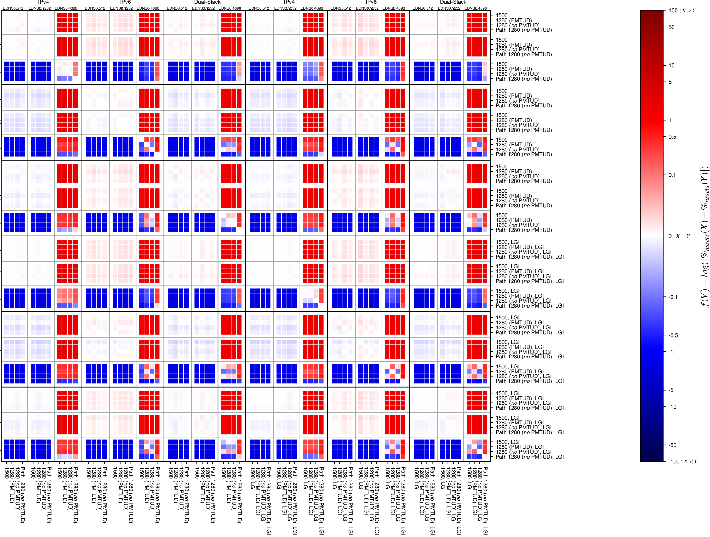
dnssec-both-UDP_frag_too_big
