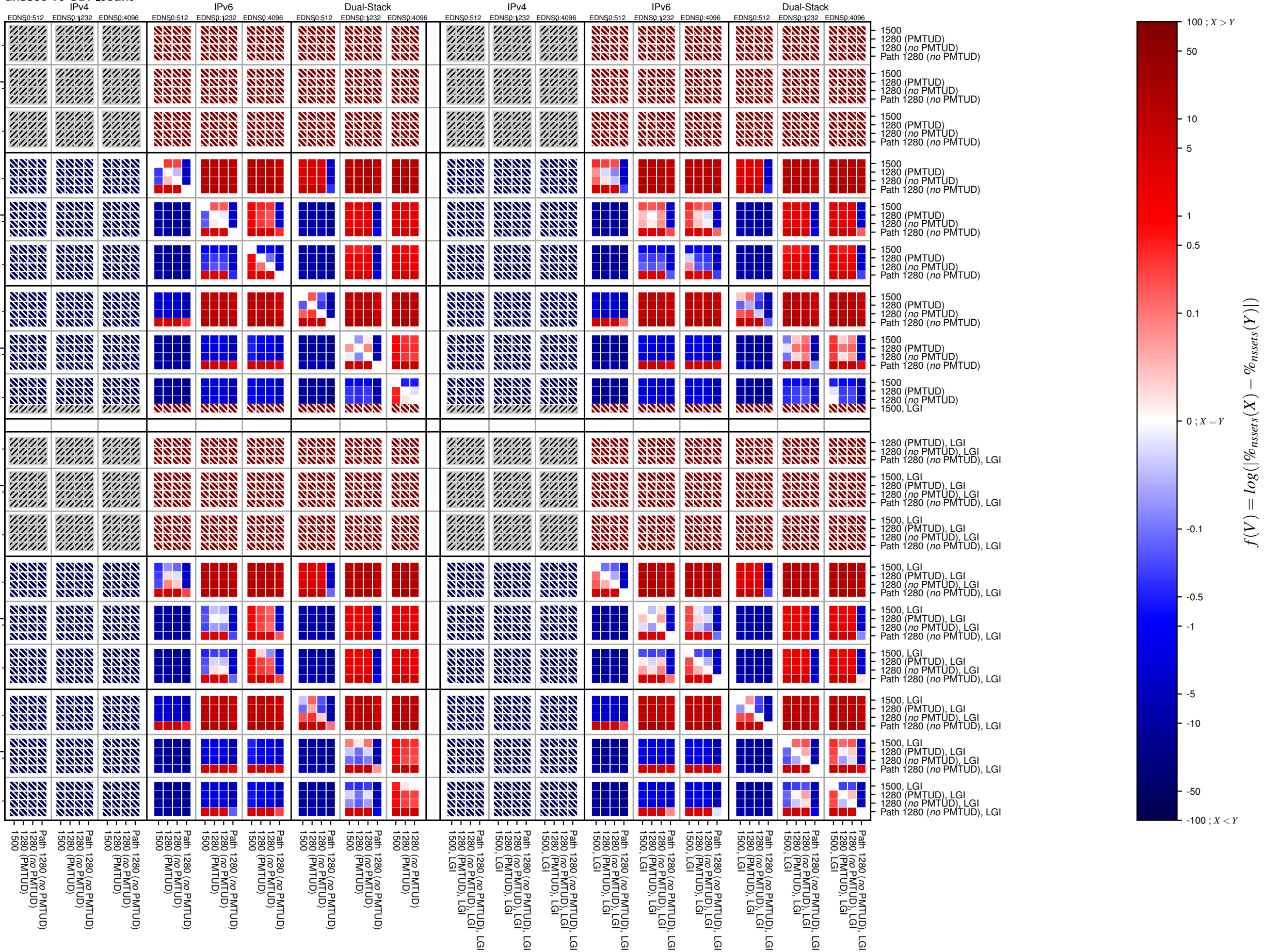
dnssec-v6-UDP_count
