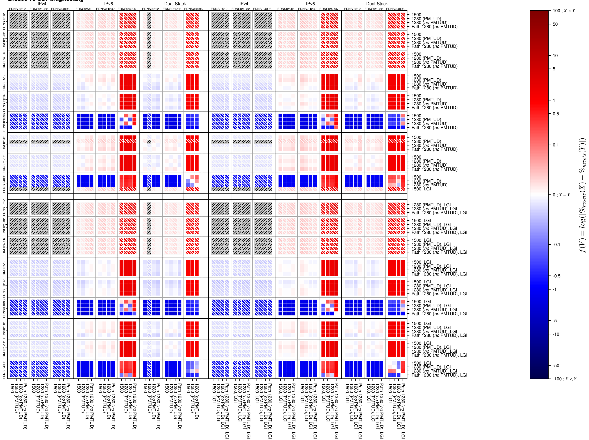
dnssec-v6-UDP_frag_too_big
