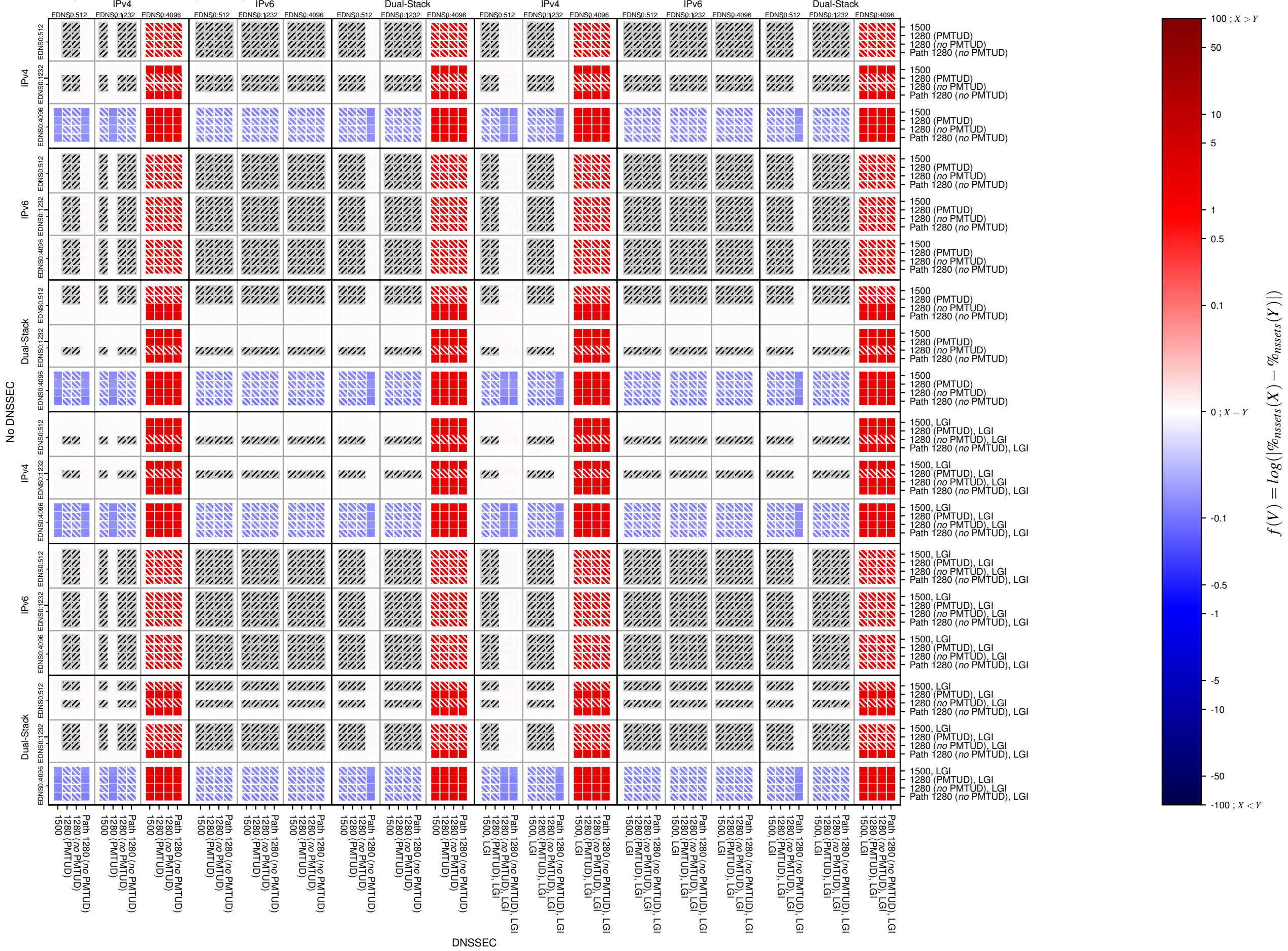
comp_dnssec-v4-UDP_frag_too_big
