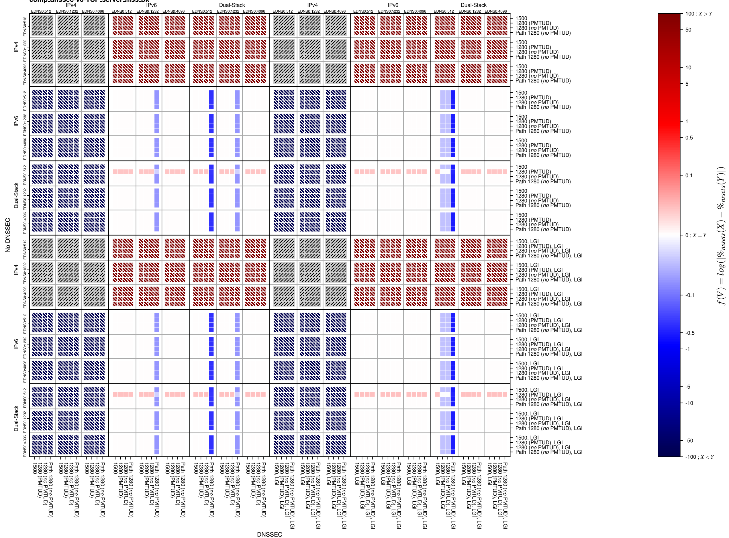
comp_dnssec-v6-TCP_server_mss_ok
