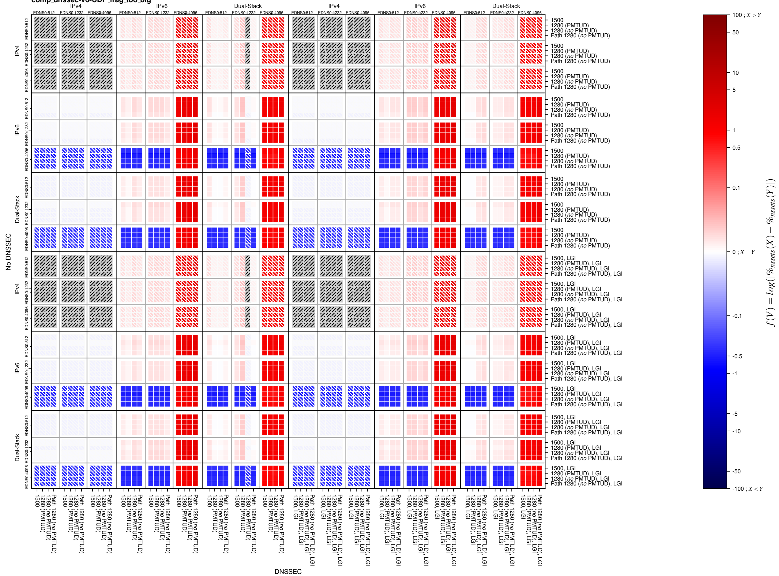
comp_dnssec-v6-UDP_frag_too_big
