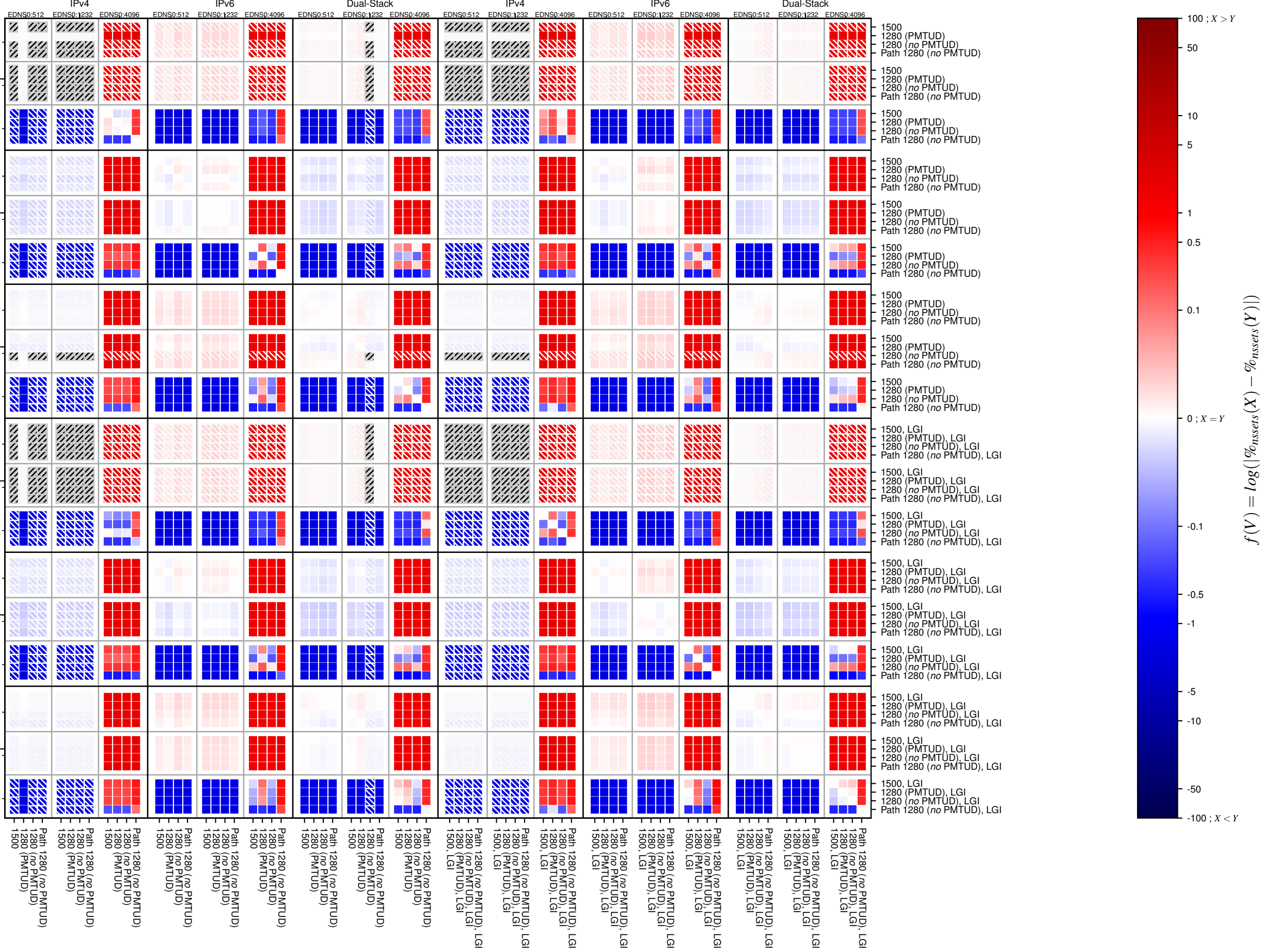
dnssec-both-UDP_frag_too_big
