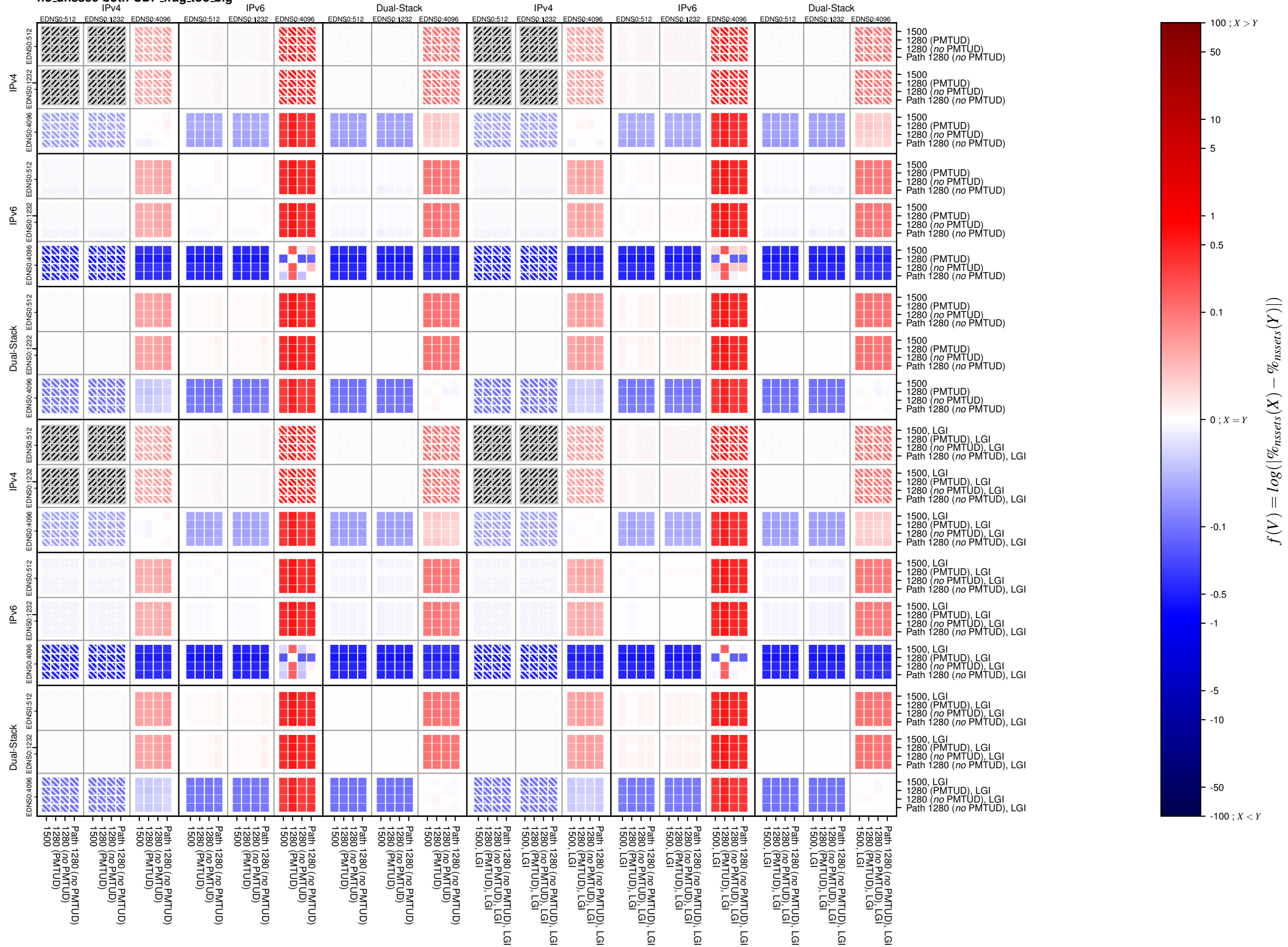
no_dnssec-both-UDP_frag_too_big
