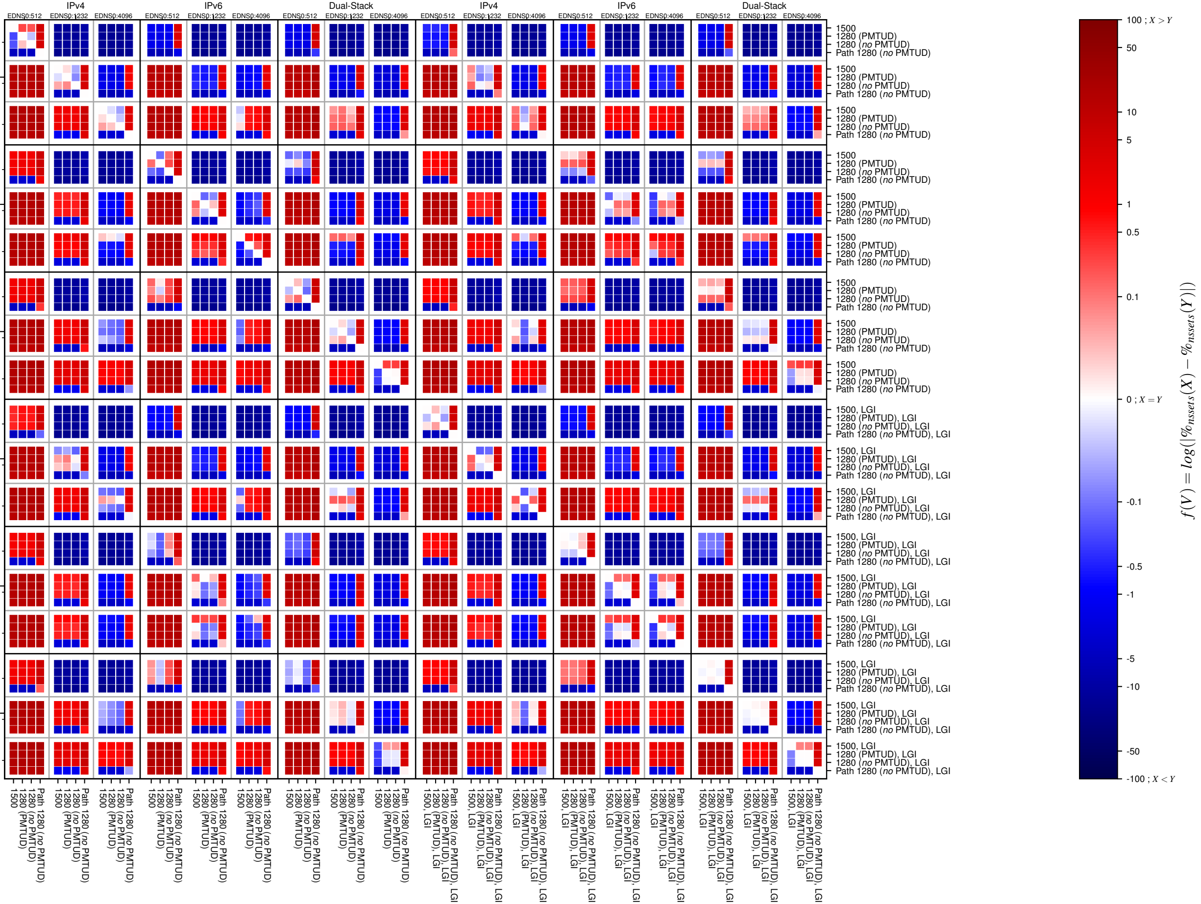
dnssec-both-TCP_count
