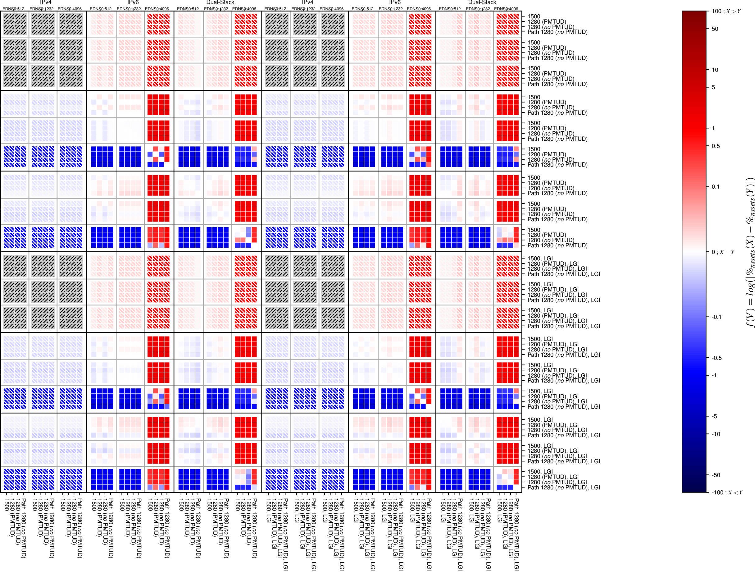
dnssec-v6-UDP_frag.too.big
