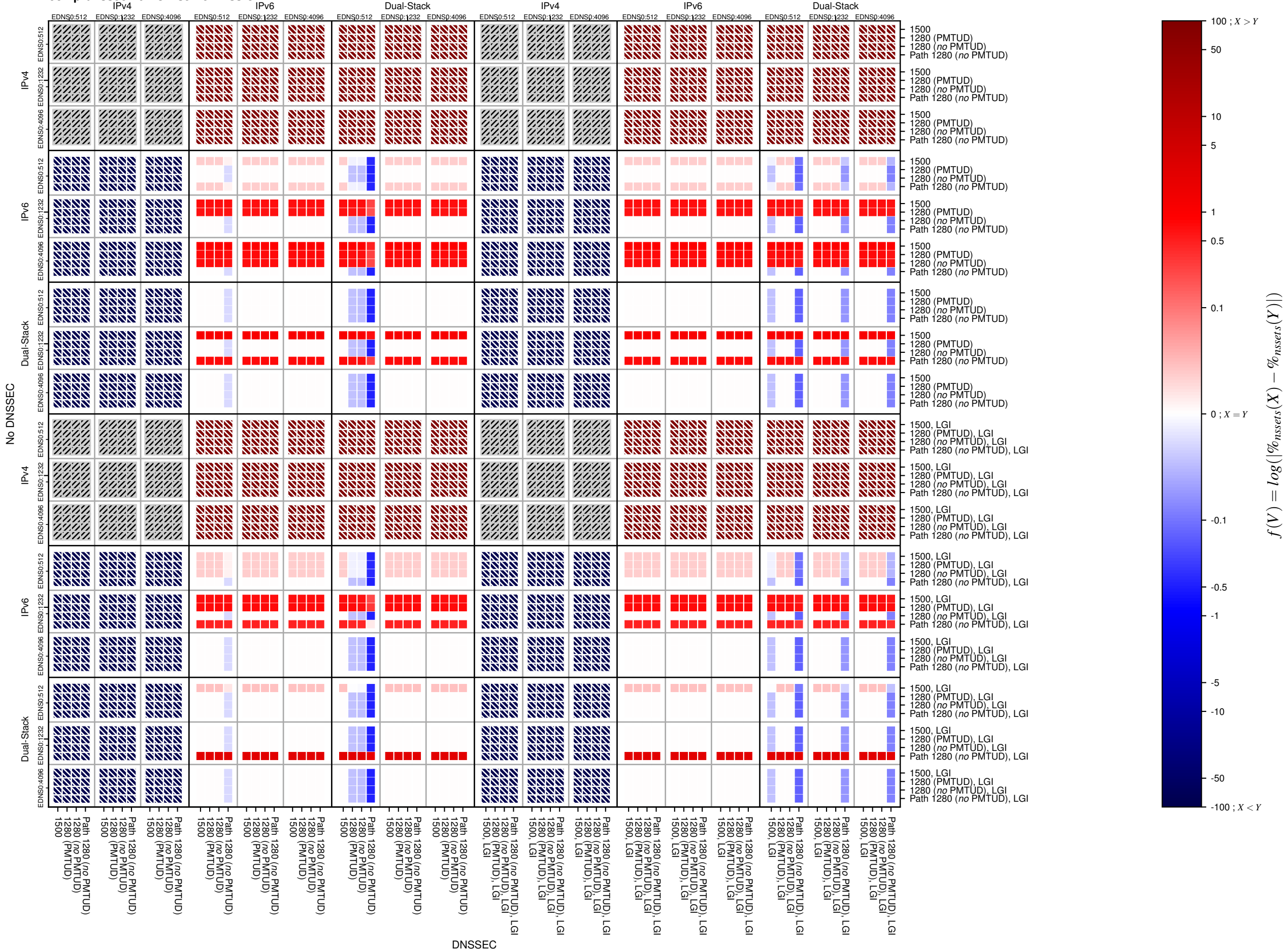
comp_dnssec-v6-TCP_server_mss_ok
