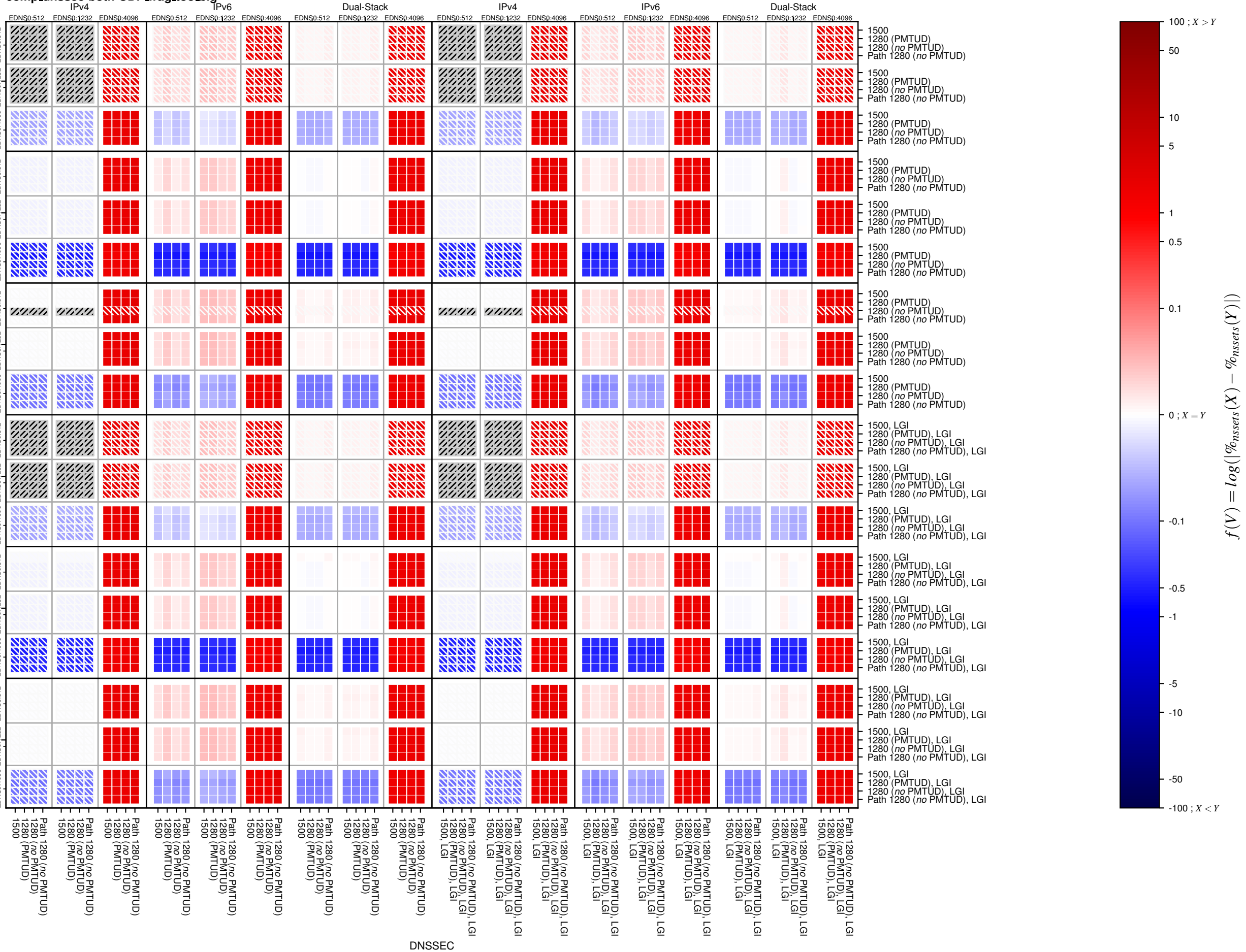
comp_dnssec-both-UDP_frag_too_big
