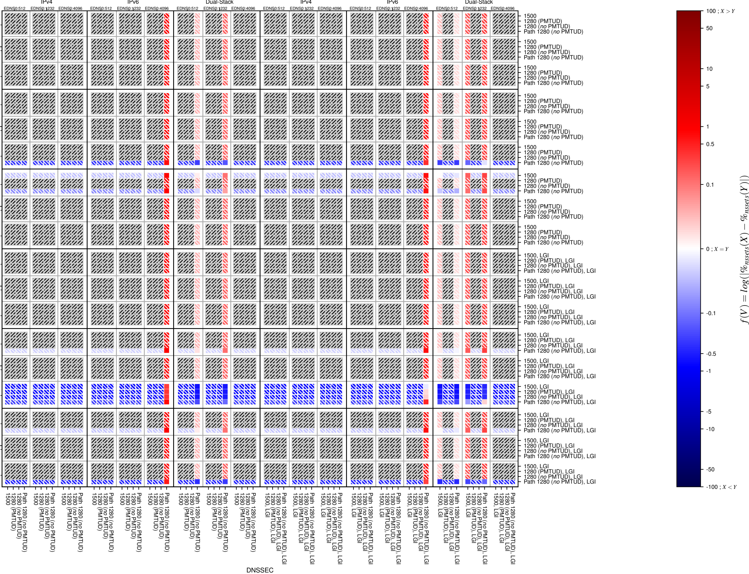
comp_dnssec-v6-TCP_frag_too_big
