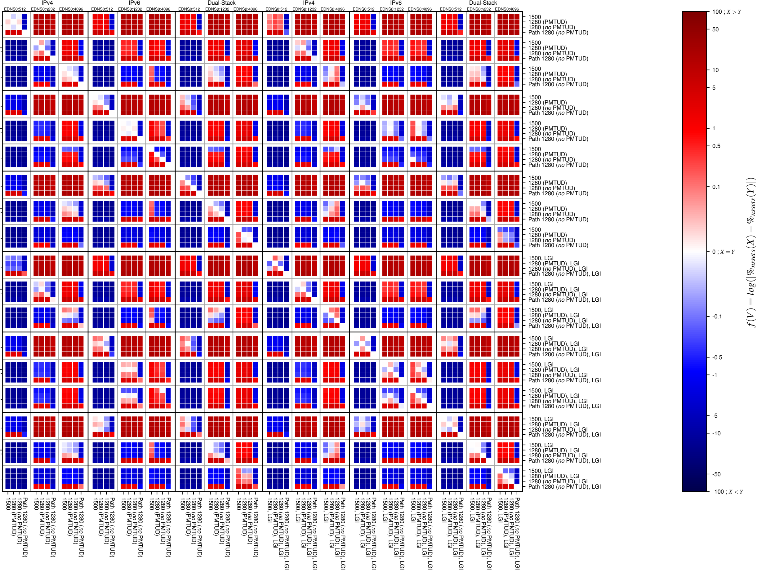
dnssec-both-UDP_count
