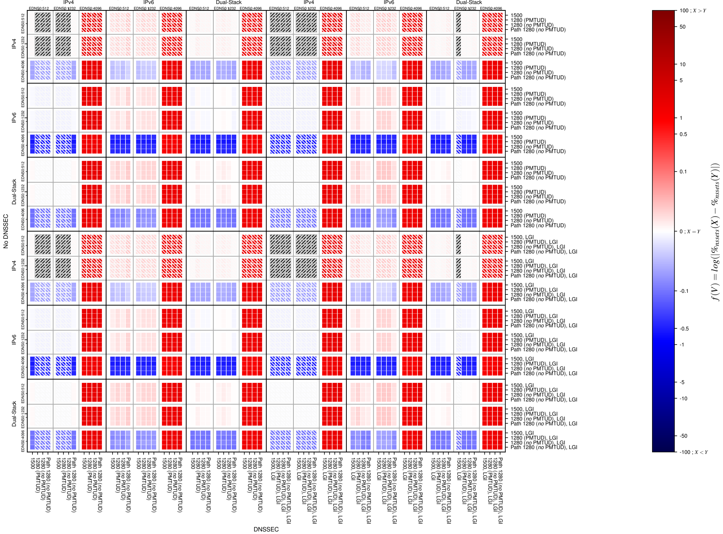
comp_dnssec-both-UDP_frag.too.big
