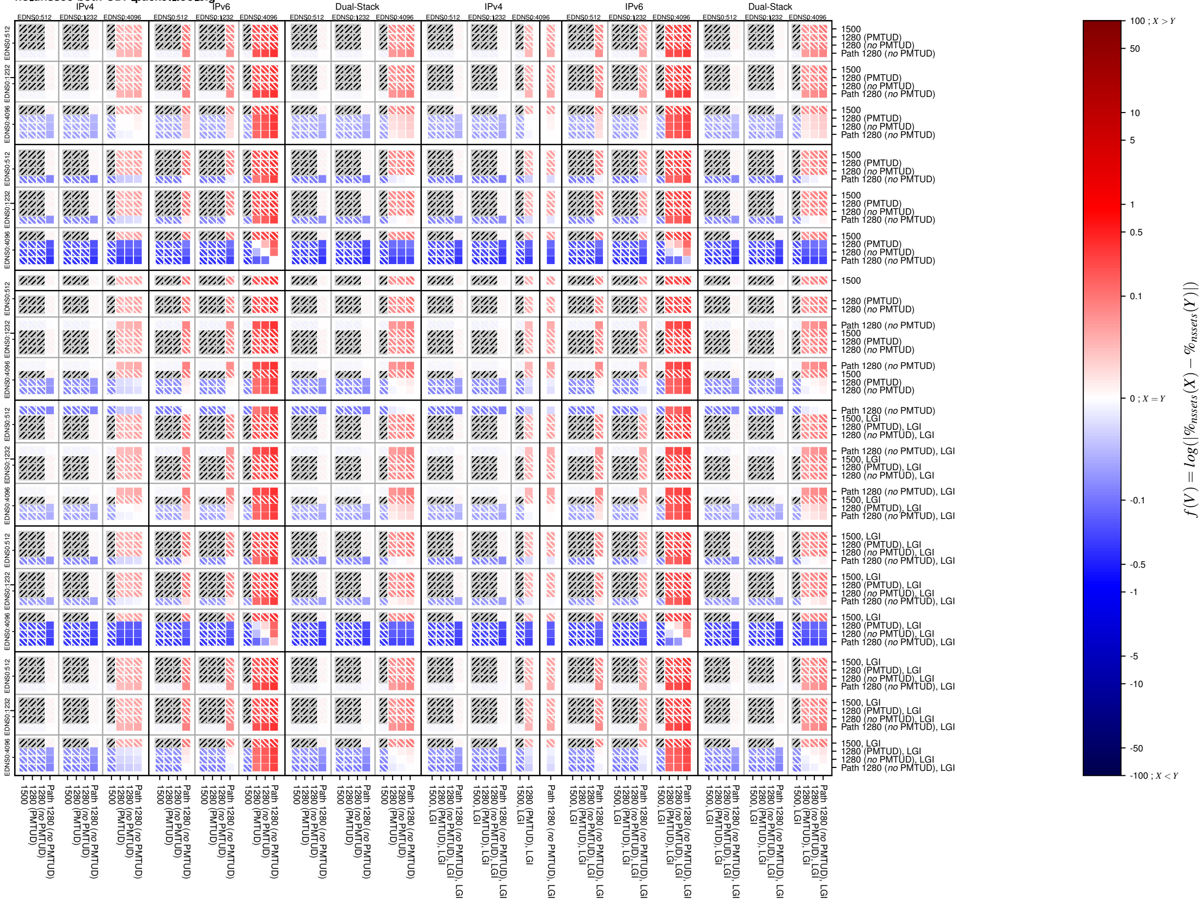
no_dnssec-both-UDP_packet_too_big
