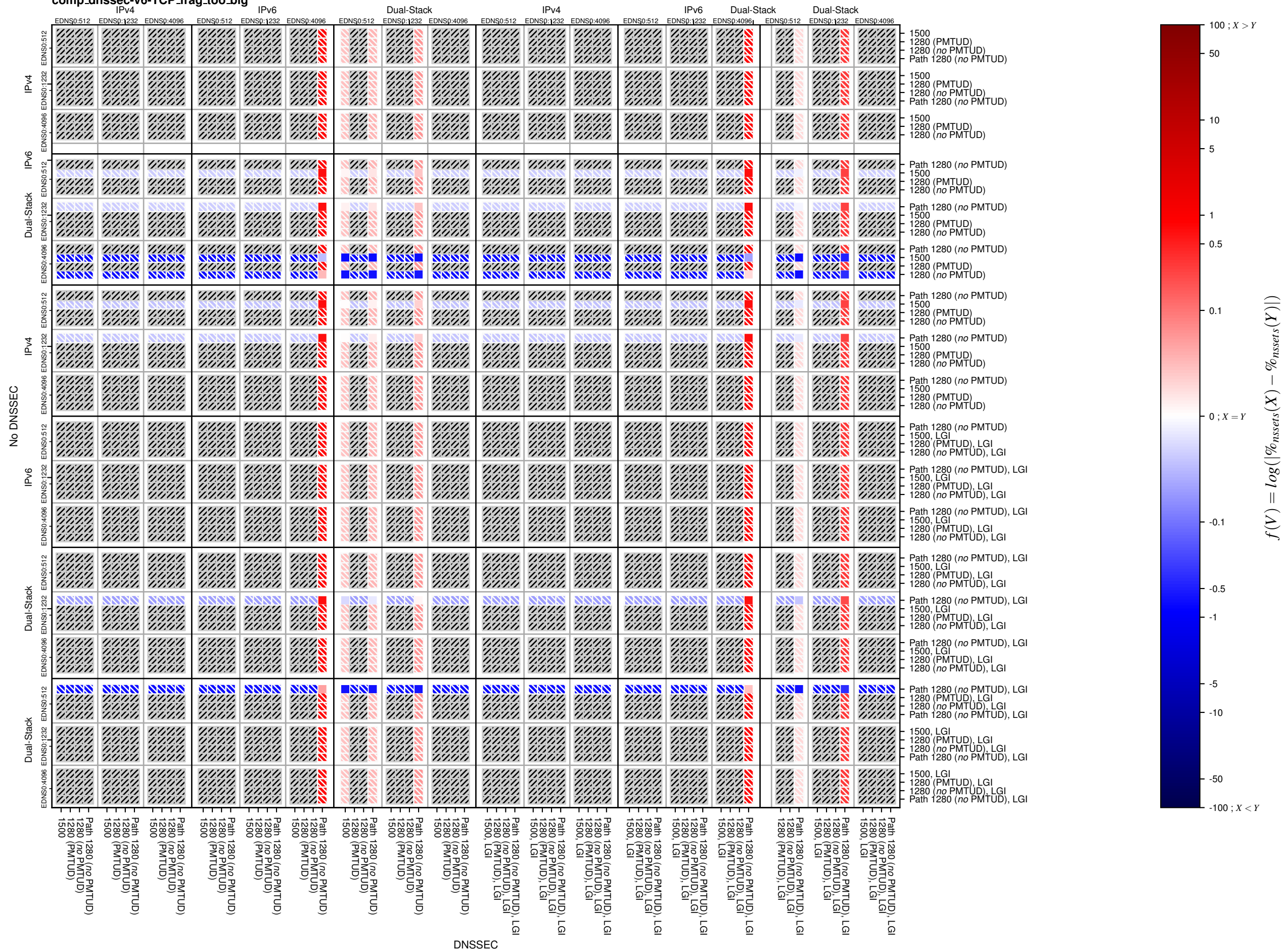
comp_dnssec-v6-TCP_frag_too_big
