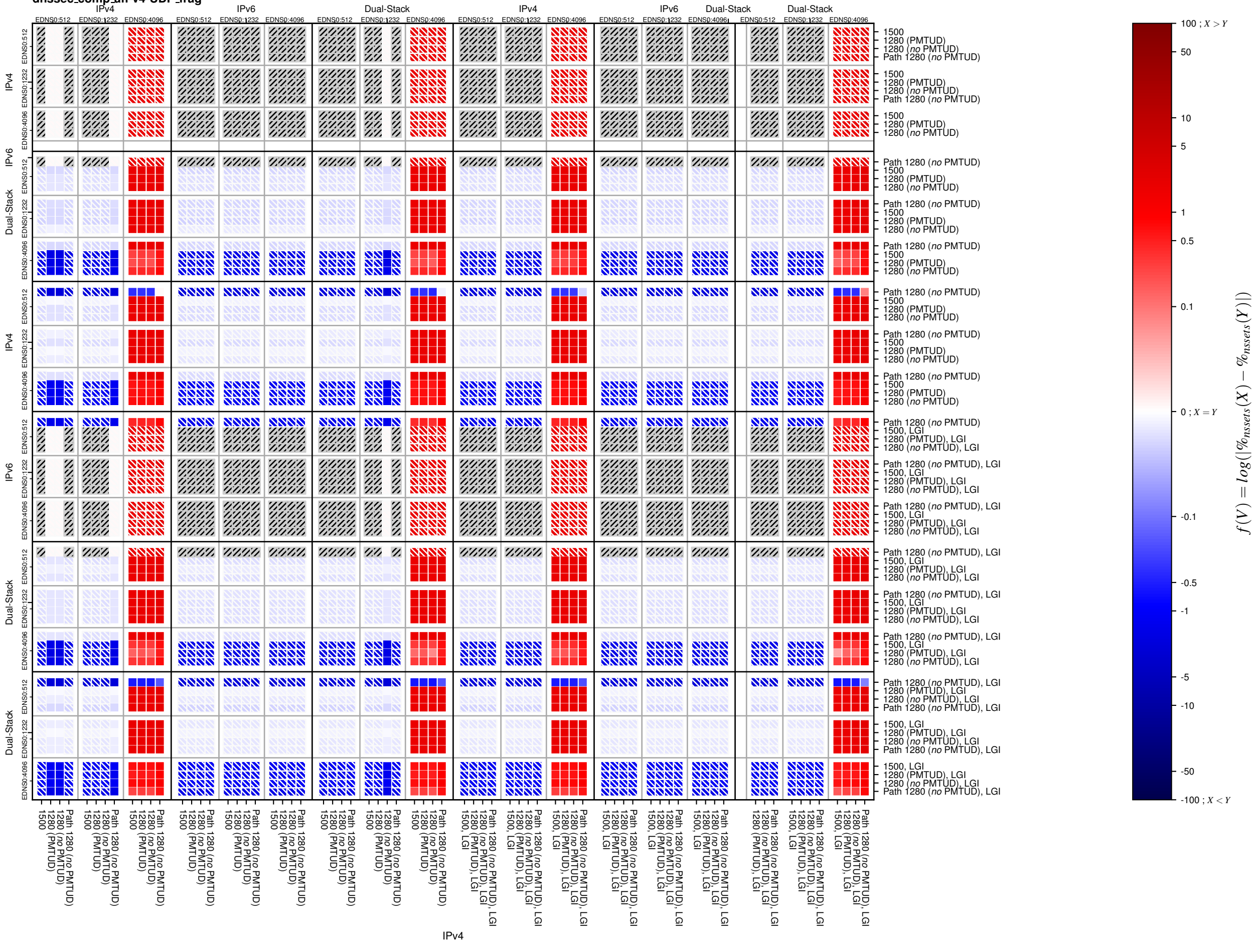
dnssec_comp_afv4-UDP_frag
