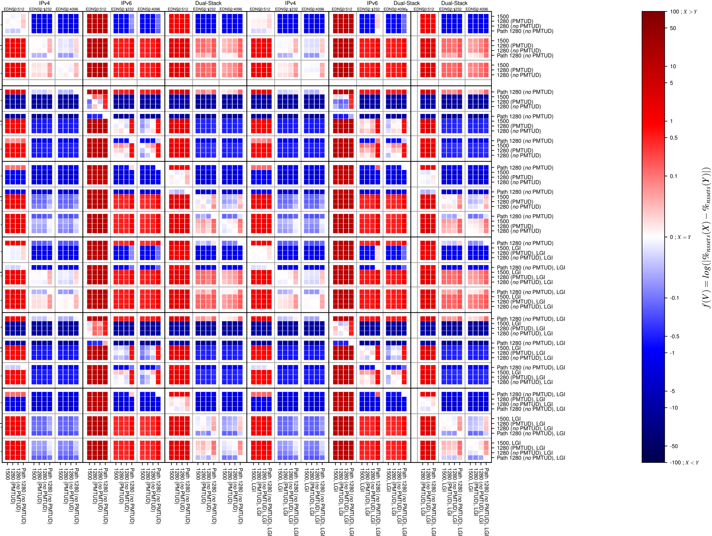
no_dnssec-both-TCP_count
