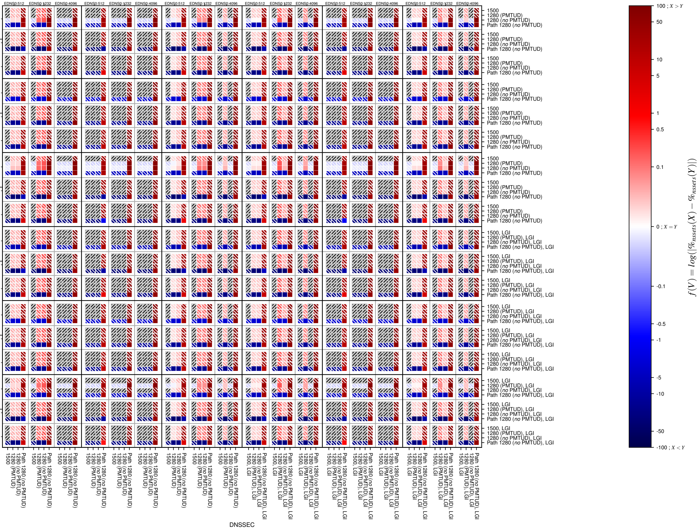
comp_dnssec-both-TCP_packet_too_big
