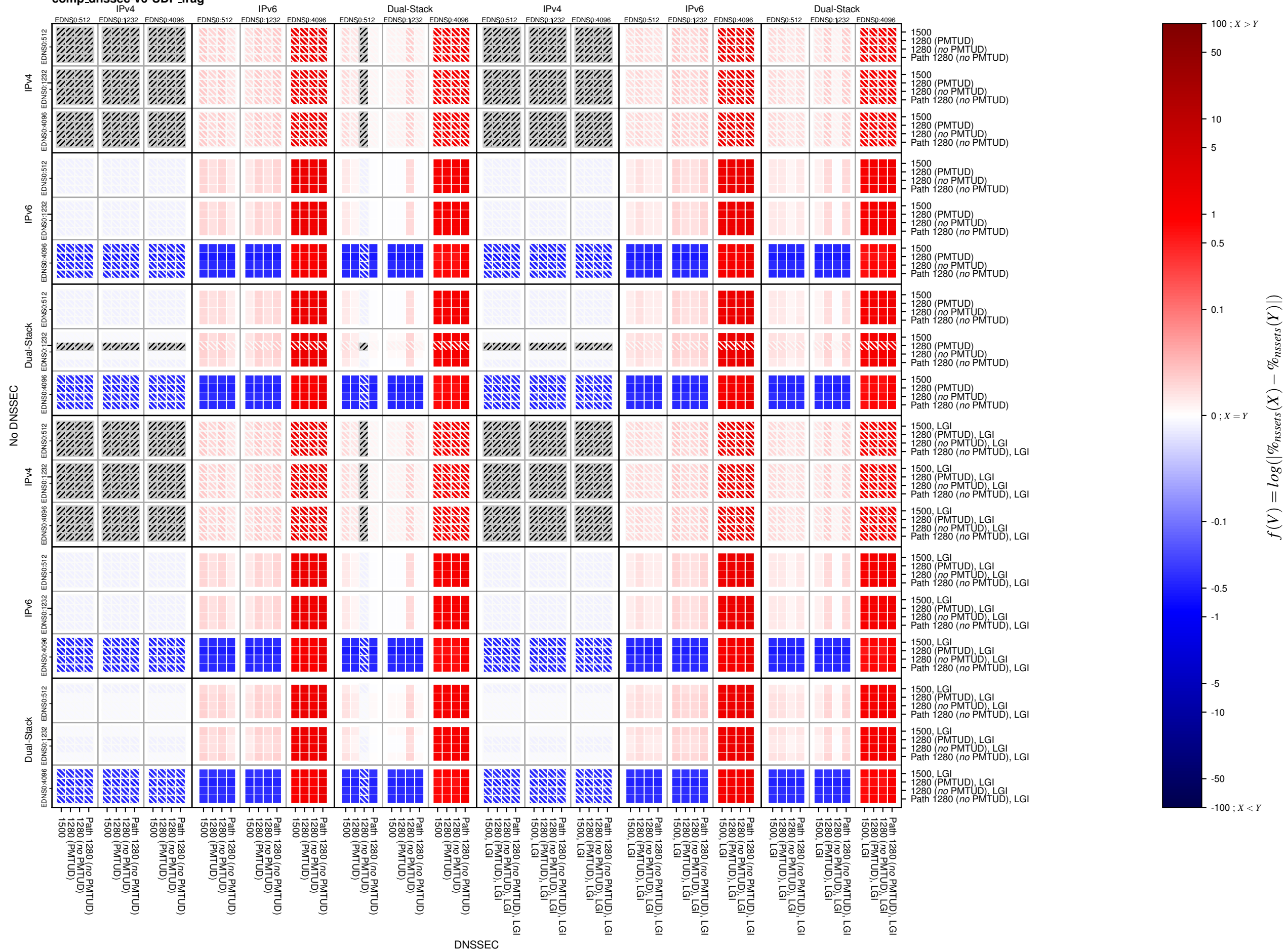
comp_dnssec-v6-UDP_frag
